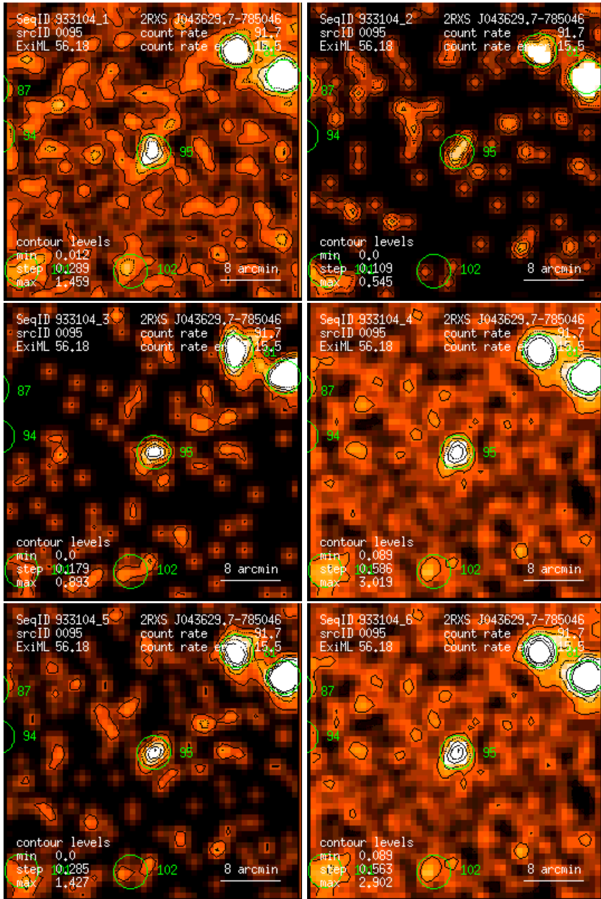
Figure 95: RASS 933104: detection 0095: band rate images, Gaussian filter: (1) PSPC channels 11 – 41, (2) 52 – 90, (3) 91 – 201, (4) 11 – 235, (5) 52 – 201, (6) 11 – 201. Broad band rates in counts/ks. Band rate contour levels in counts/ks/arcmin 2 .
