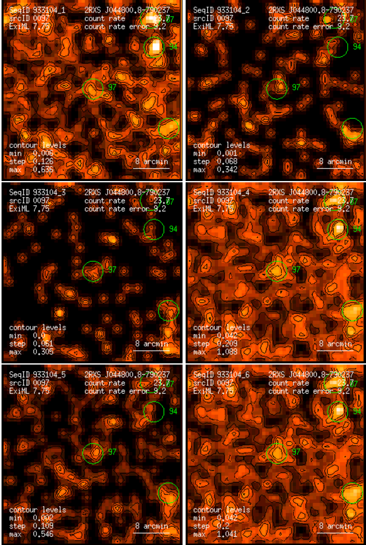
Figure 97: RASS 933104: detection 0097: band rate images, Gaussian filter: (1) PSPC channels 11 – 41, (2) 52 – 90, (3) 91 – 201, (4) 11 – 235, (5) 52 – 201, (6) 11 – 201. Broad band rates in counts/ks. Band rate contour levels in counts/ks/arcmin 2 .
