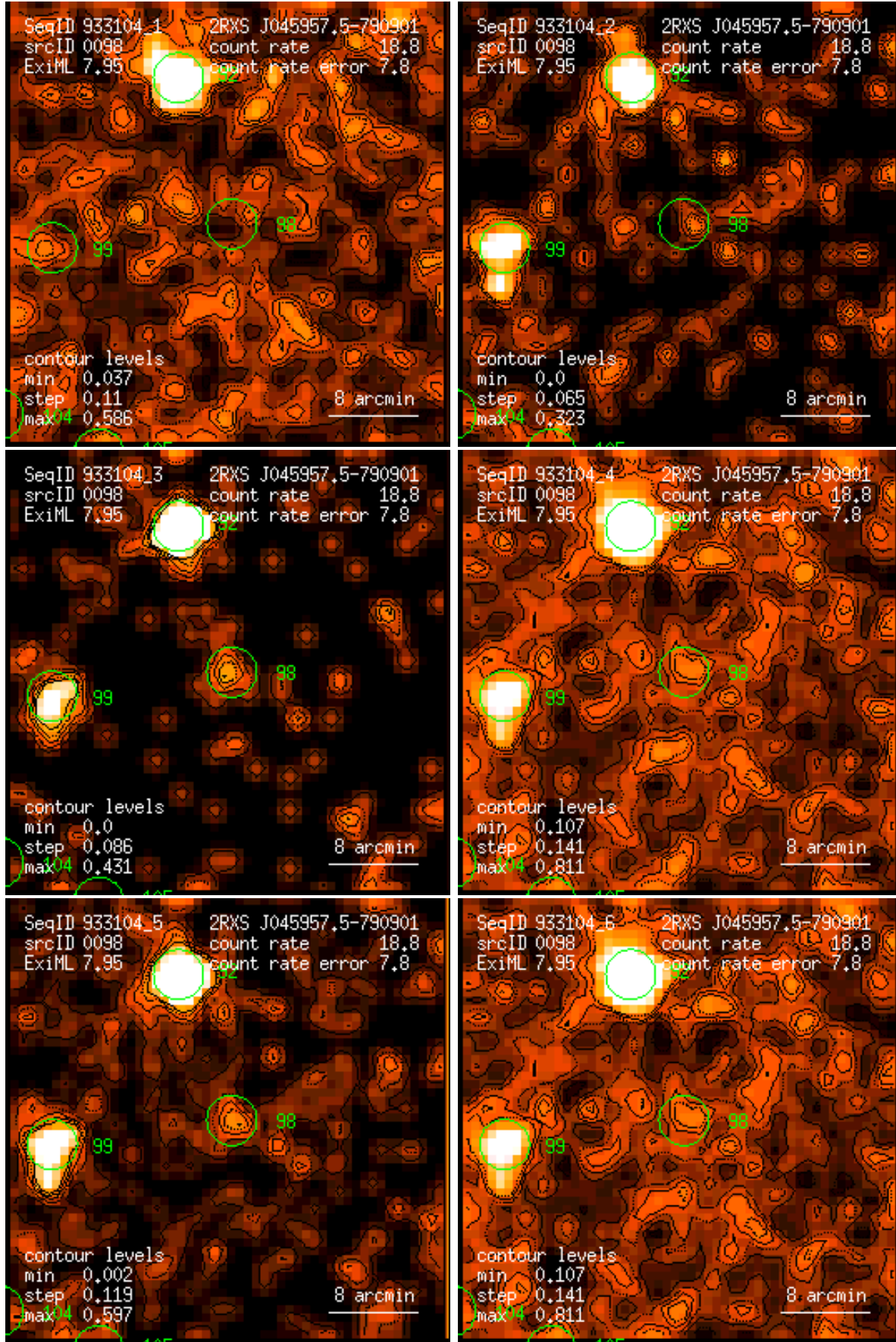
Figure 98: RASS 933104: detection 0098: band rate images, Gaussian filter: (1) PSPC channels 11 – 41, (2) 52 – 90, (3) 91 – 201, (4) 11 – 235, (5) 52 – 201, (6) 11 – 201. Broad band rates in counts/ks. Band rate contour levels in counts/ks/arcmin 2 .
