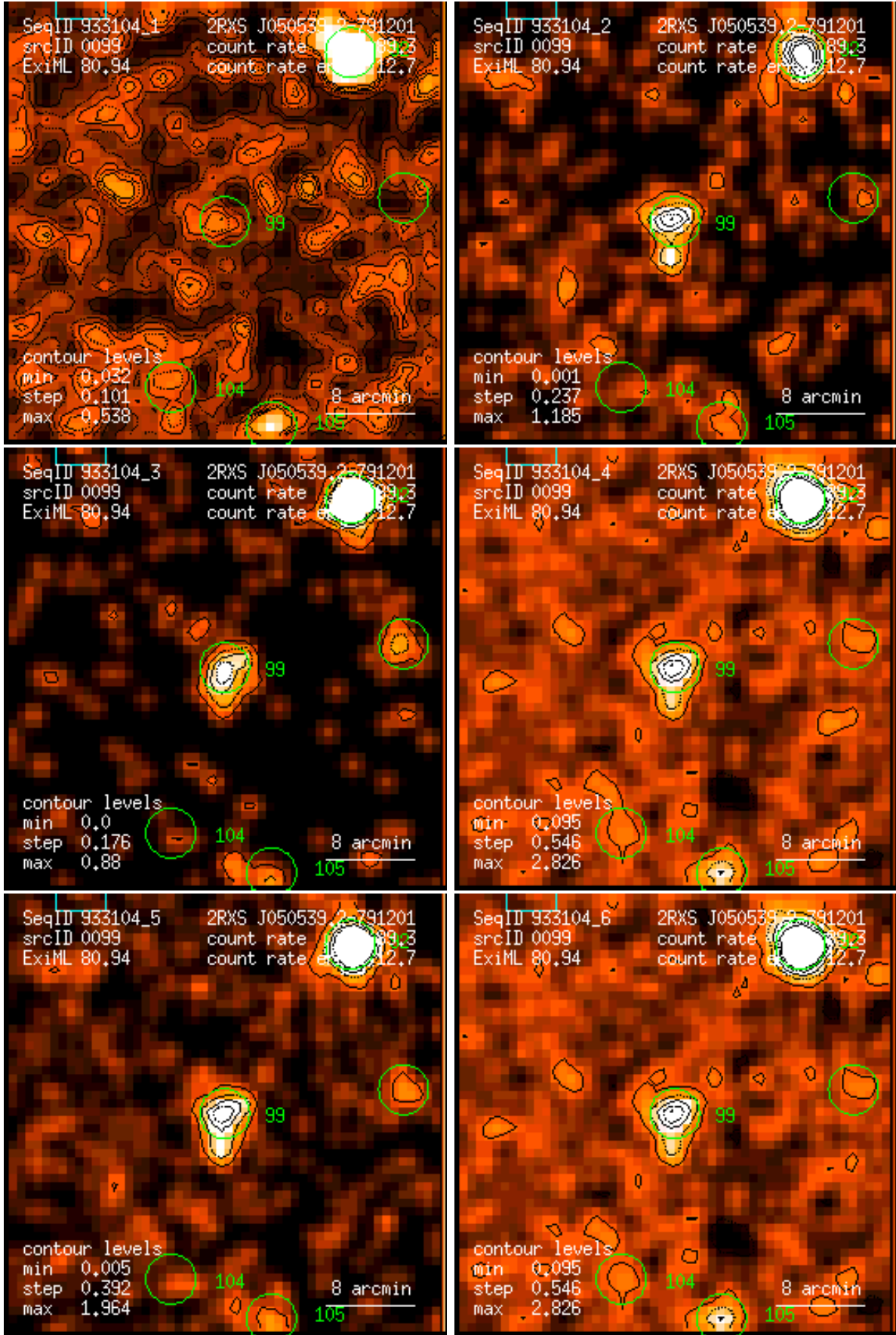
Figure 99: RASS 933104: detection 0099: band rate images, Gaussian filter: (1) PSPC channels 11 – 41, (2) 52 – 90, (3) 91 – 201, (4) 11 – 235, (5) 52 – 201, (6) 11 – 201. Broad band rates in counts/ks. Band rate contour levels in counts/ks/arcmin 2 .
