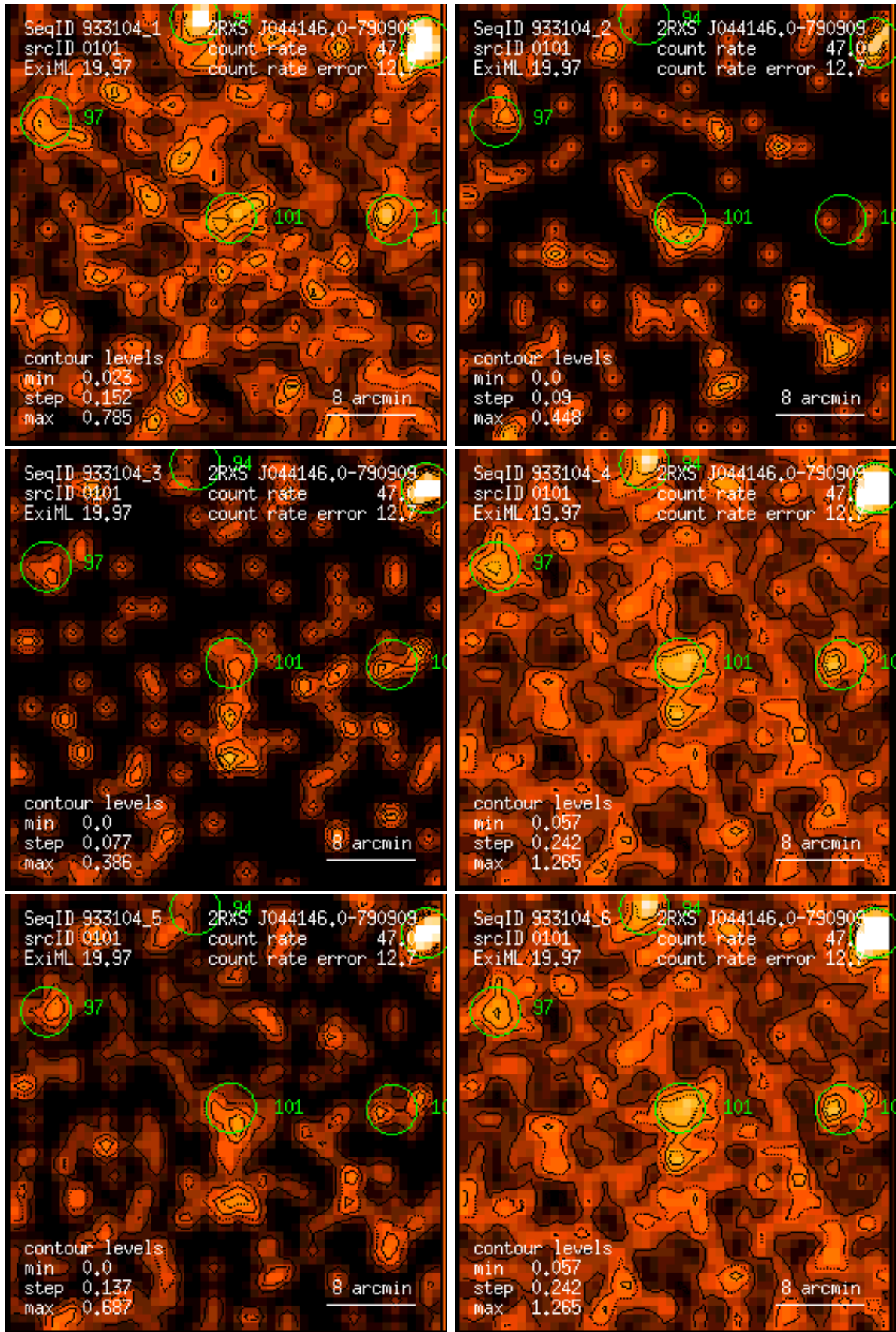
Figure 101: RASS 933104: detection 0101: band rate images, Gaussian filter: (1) PSPC channels 11 – 41, (2) 52 – 90, (3) 91 – 201, (4) 11 – 235, (5) 52 – 201, (6) 11 – 201. Broad band rates in counts/ks. Band rate contour levels in counts/ks/arcmin 2 .
