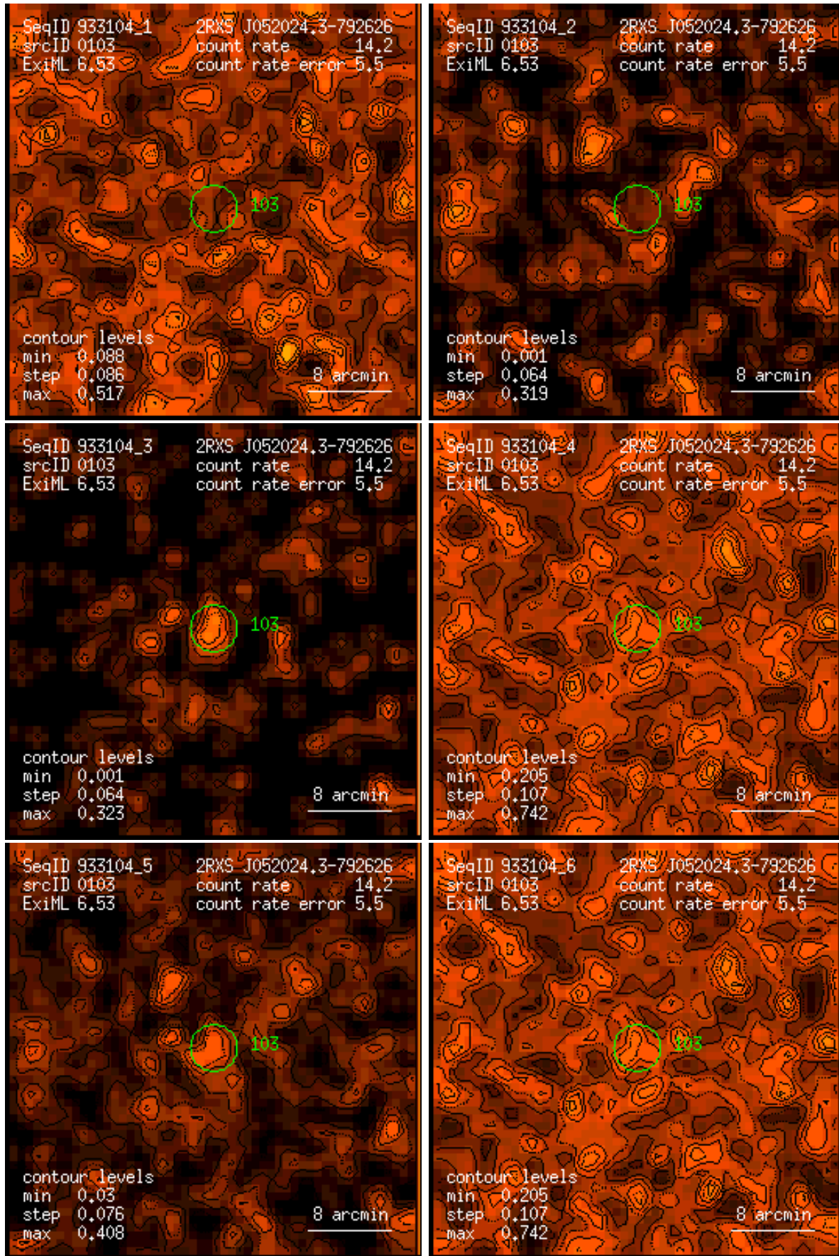
Figure 103: RASS 933104: detection 0103: band rate images, Gaussian filter: (1) PSPC channels 11 – 41, (2) 52 – 90, (3) 91 – 201, (4) 11 – 235, (5) 52 – 201, (6) 11 – 201. Broad band rates in counts/ks. Band rate contour levels in counts/ks/arcmin 2 .
