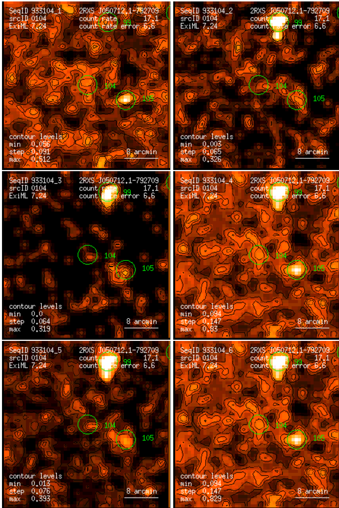
Figure 104: RASS 933104: detection 0104: band rate images, Gaussian filter: (1) PSPC channels 11 – 41, (2) 52 – 90, (3) 91 – 201, (4) 11 – 235, (5) 52 – 201, (6) 11 – 201. Broad band rates in counts/ks. Band rate contour levels in counts/ks/arcmin 2 .
