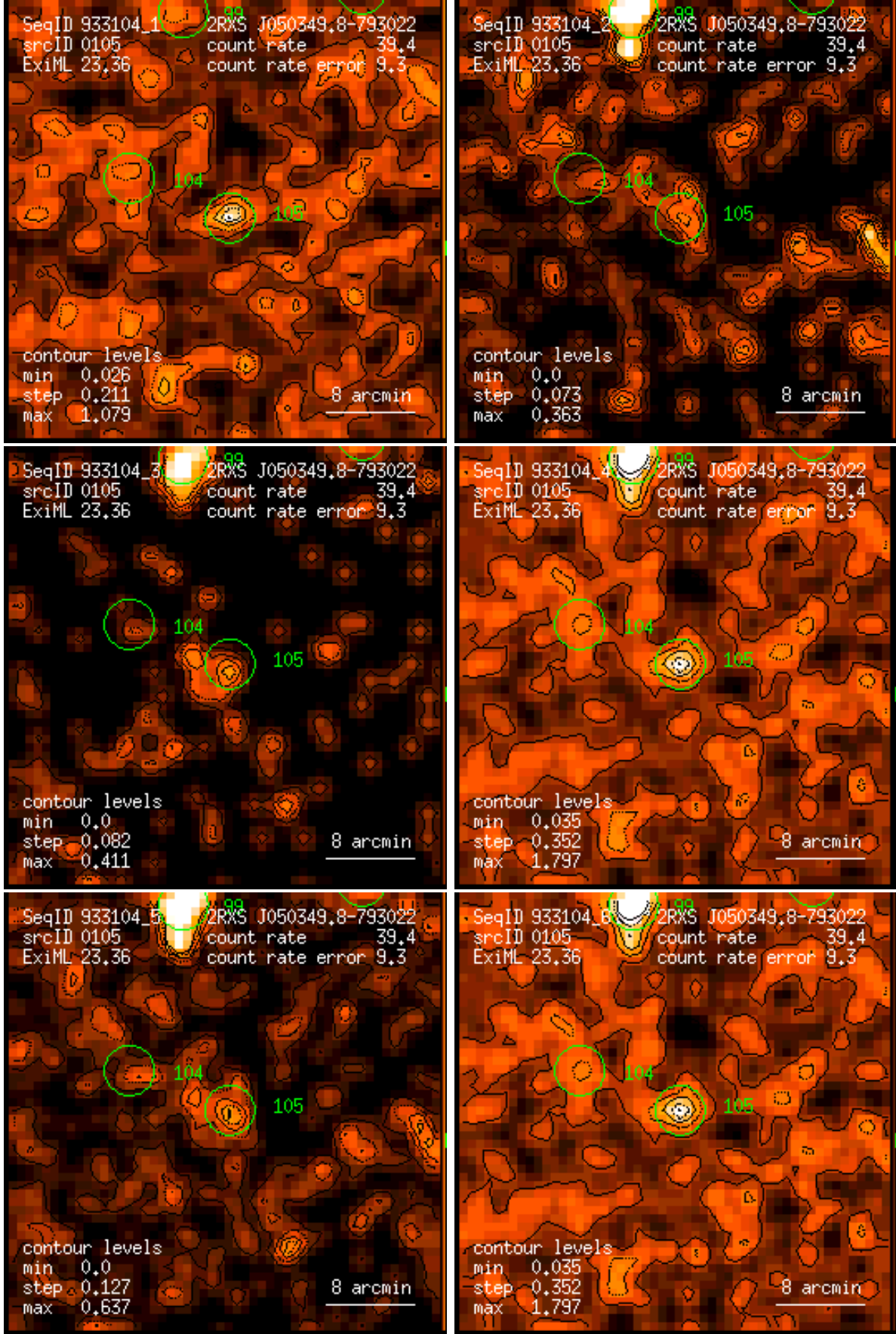
Figure 105: RASS 933104: detection 0105: band rate images, Gaussian filter: (1) PSPC channels 11 – 41, (2) 52 – 90, (3) 91 – 201, (4) 11 – 235, (5) 52 – 201, (6) 11 – 201. Broad band rates in counts/ks. Band rate contour levels in counts/ks/arcmin 2 .
