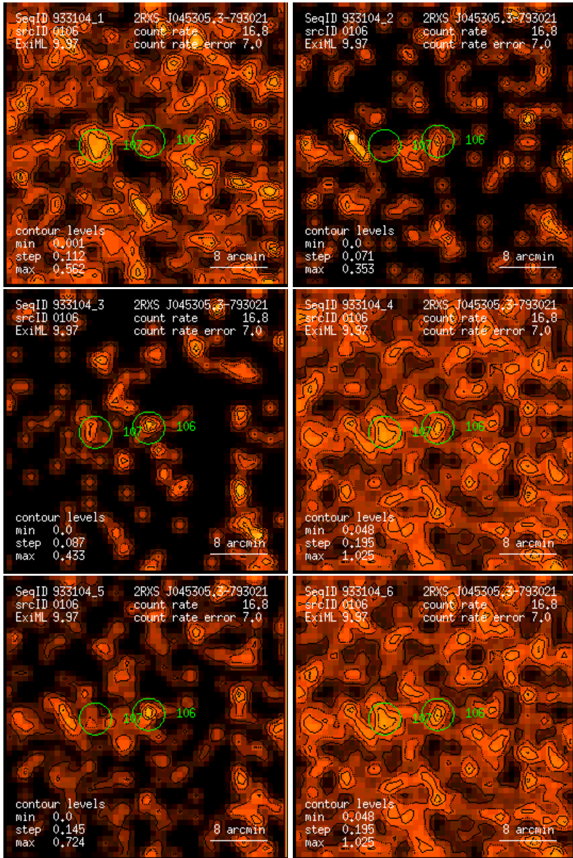
Figure 106: RASS 933104: detection 0106: band rate images, Gaussian filter: (1) PSPC channels 11 – 41, (2) 52 – 90, (3) 91 – 201, (4) 11 – 235, (5) 52 – 201, (6) 11 – 201. Broad band rates in counts/ks. Band rate contour levels in counts/ks/arcmin 2 .
