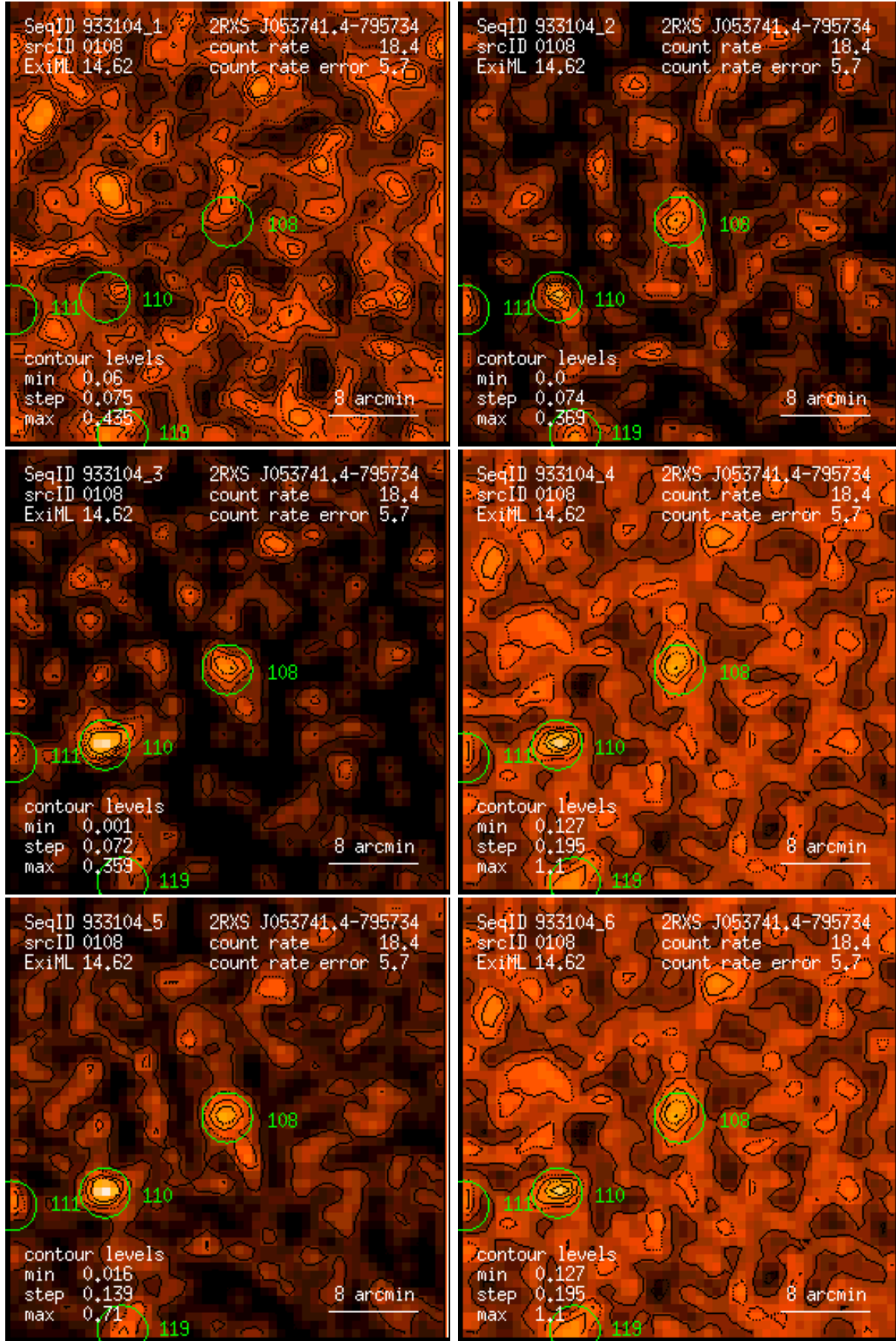
Figure 108: RASS 933104: detection 0108: band rate images, Gaussian filter: (1) PSPC channels 11 – 41, (2) 52 – 90, (3) 91 – 201, (4) 11 – 235, (5) 52 – 201, (6) 11 – 201. Broad band rates in counts/ks. Band rate contour levels in counts/ks/arcmin 2 .
