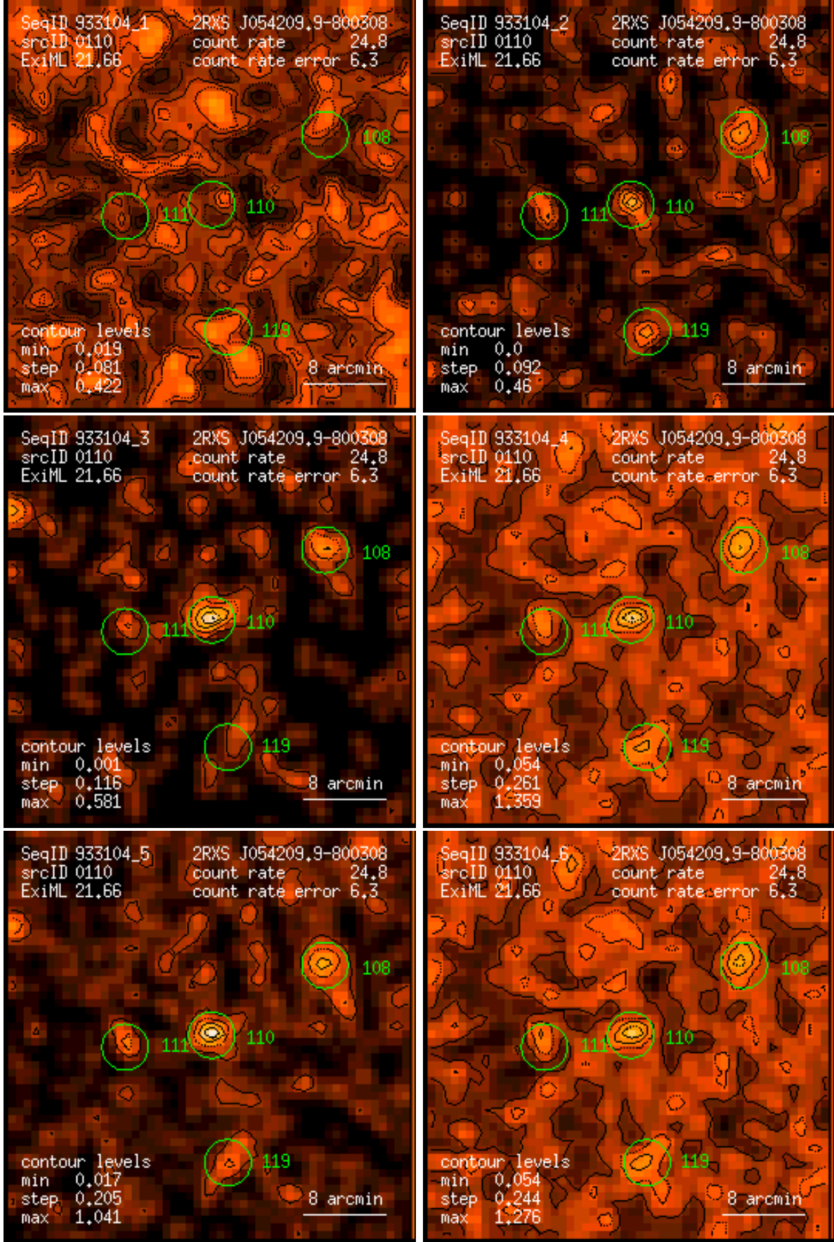
Figure 110: RASS 933104: detection 0110: band rate images, Gaussian filter: (1) PSPC channels 11 – 41, (2) 52 – 90, (3) 91 – 201, (4) 11 – 235, (5) 52 – 201, (6) 11 – 201. Broad band rates in counts/ks. Band rate contour levels in counts/ks/arcmin 2 .
