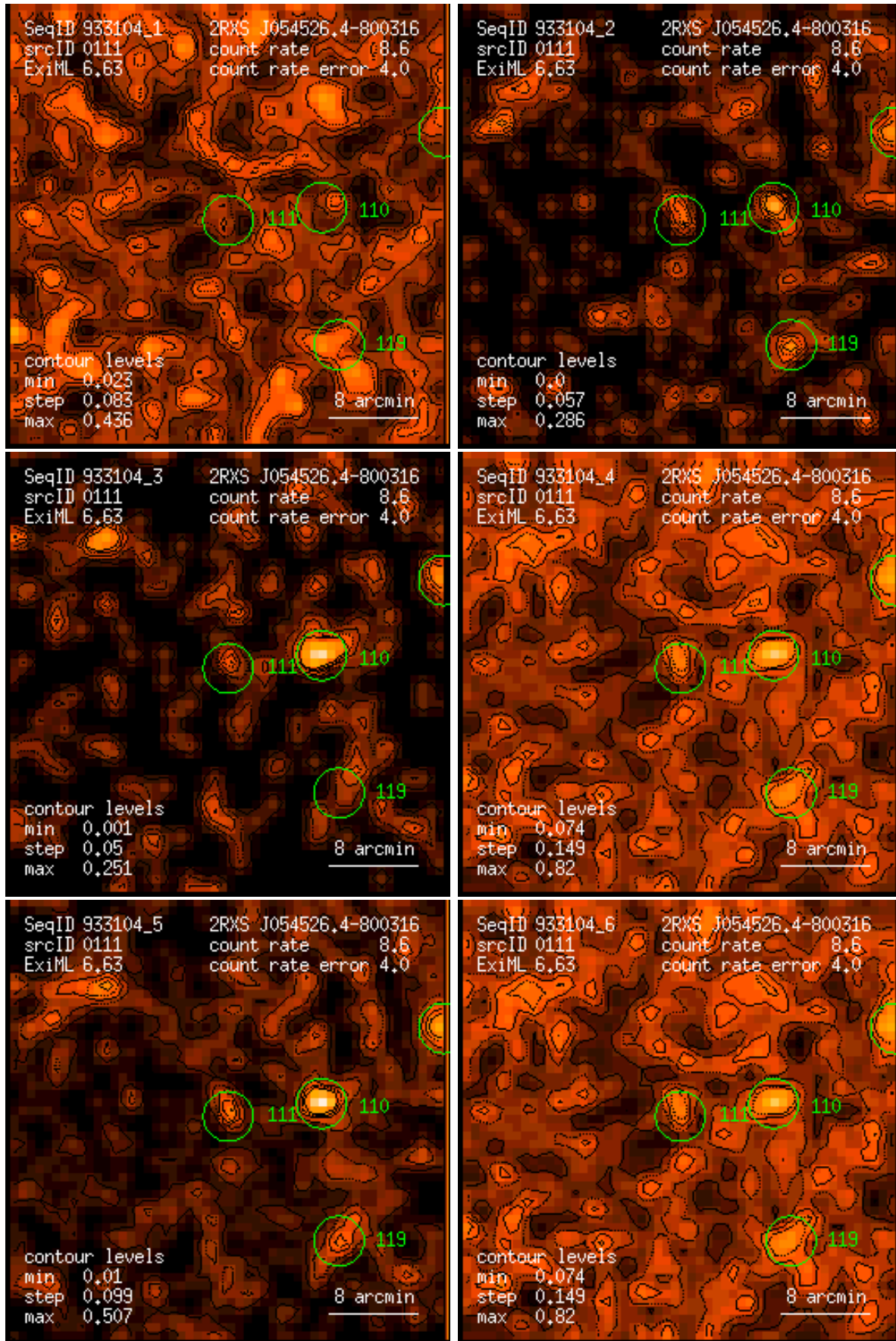
Figure 111: RASS 933104: detection 0111: band rate images, Gaussian filter: (1) PSPC channels 11 – 41, (2) 52 – 90, (3) 91 – 201, (4) 11 – 235, (5) 52 – 201, (6) 11 – 201. Broad band rates in counts/ks. Band rate contour levels in counts/ks/arcmin 2 .
