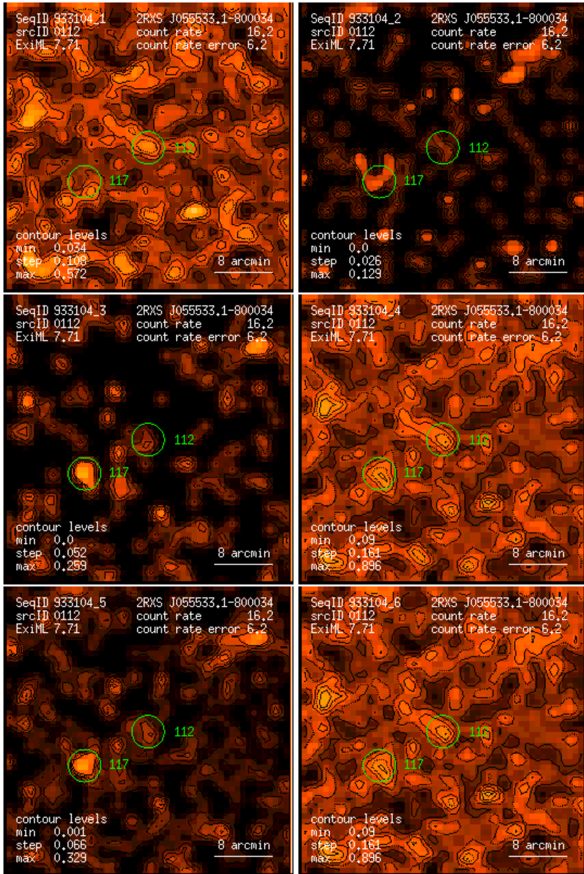
Figure 112: RASS 933104: detection 0112: band rate images, Gaussian filter: (1) PSPC channels 11 – 41, (2) 52 – 90, (3) 91 – 201, (4) 11 – 235, (5) 52 – 201, (6) 11 – 201. Broad band rates in counts/ks. Band rate contour levels in counts/ks/arcmin 2 .
