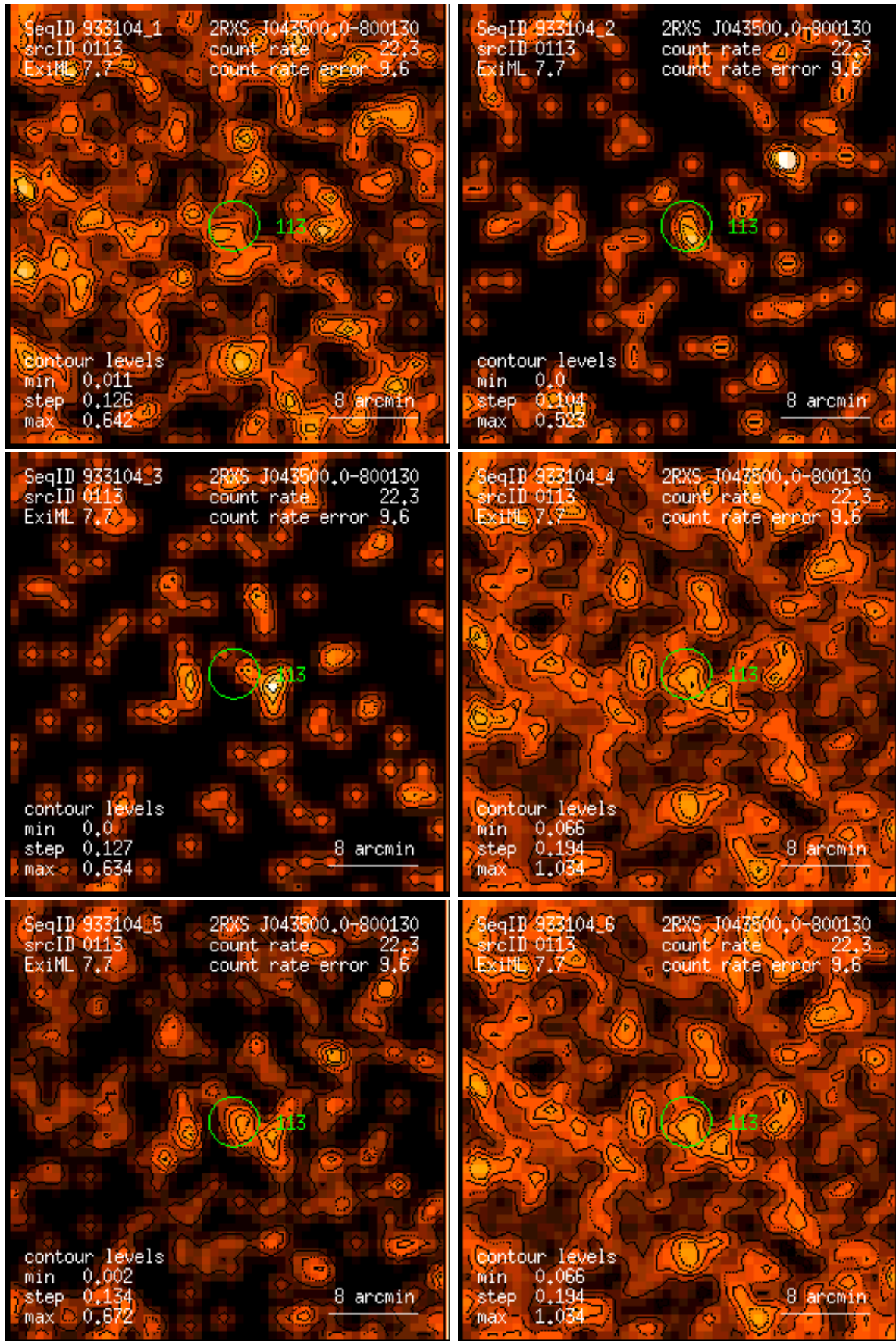
Figure 113: RASS 933104: detection 0113: band rate images, Gaussian filter: (1) PSPC channels 11 – 41, (2) 52 – 90, (3) 91 – 201, (4) 11 – 235, (5) 52 – 201, (6) 11 – 201. Broad band rates in counts/ks. Band rate contour levels in counts/ks/arcmin 2 .
