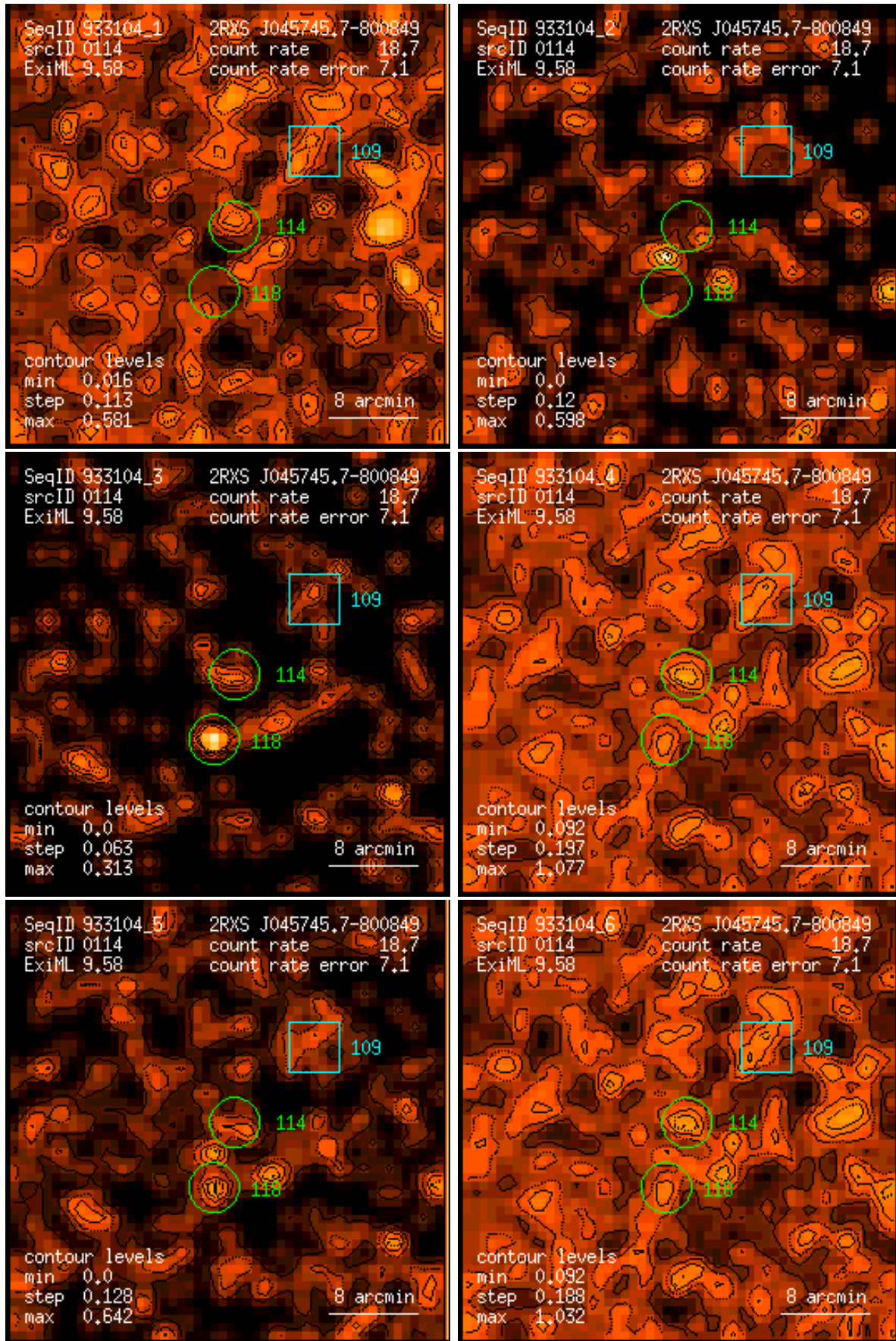
Figure 114: RASS 933104: detection 0114: band rate images, Gaussian filter: (1) PSPC channels 11 – 41, (2) 52 – 90, (3) 91 – 201, (4) 11 – 235, (5) 52 – 201, (6) 11 – 201. Broad band rates in counts/ks. Band rate contour levels in counts/ks/arcmin 2 .
