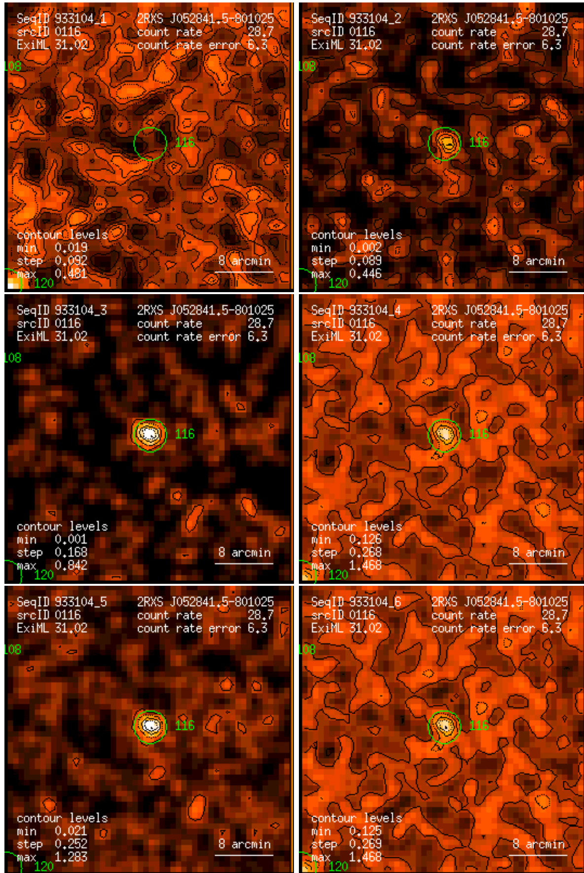
Figure 116: RASS 933104: detection 0116: band rate images, Gaussian filter: (1) PSPC channels 11 – 41, (2) 52 – 90, (3) 91 – 201, (4) 11 – 235, (5) 52 – 201, (6) 11 – 201. Broad band rates in counts/ks. Band rate contour levels in counts/ks/arcmin 2 .
