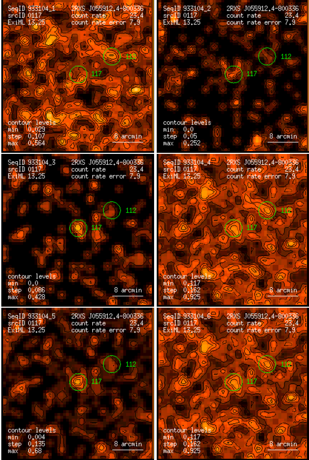
Figure 117: RASS 933104: detection 0117: band rate images, Gaussian filter: (1) PSPC channels 11 – 41, (2) 52 – 90, (3) 91 – 201, (4) 11 – 235, (5) 52 – 201, (6) 11 – 201. Broad band rates in counts/ks. Band rate contour levels in counts/ks/arcmin 2 .
