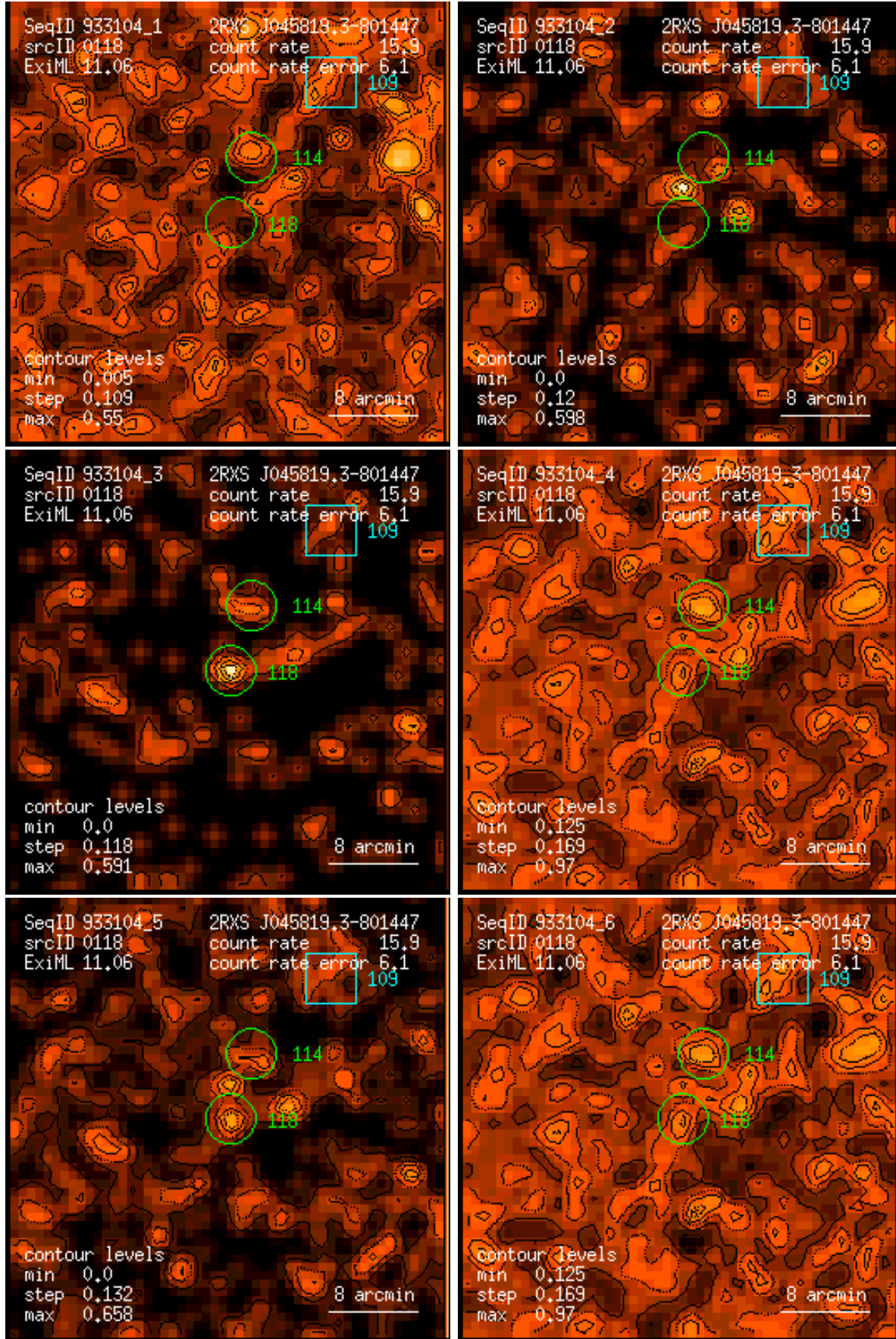
Figure 118: RASS 933104: detection 0118: band rate images, Gaussian filter: (1) PSPC channels 11 – 41, (2) 52 – 90, (3) 91 – 201, (4) 11 – 235, (5) 52 – 201, (6) 11 – 201. Broad band rates in counts/ks. Band rate contour levels in counts/ks/arcmin 2 .
