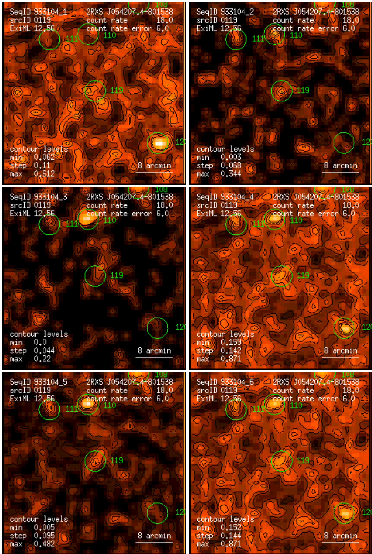
Figure 119: RASS 933104: detection 0119: band rate images, Gaussian filter: (1) PSPC channels 11 – 41, (2) 52 – 90, (3) 91 – 201, (4) 11 – 235, (5) 52 – 201, (6) 11 – 201. Broad band rates in counts/ks. Band rate contour levels in counts/ks/arcmin 2 .
