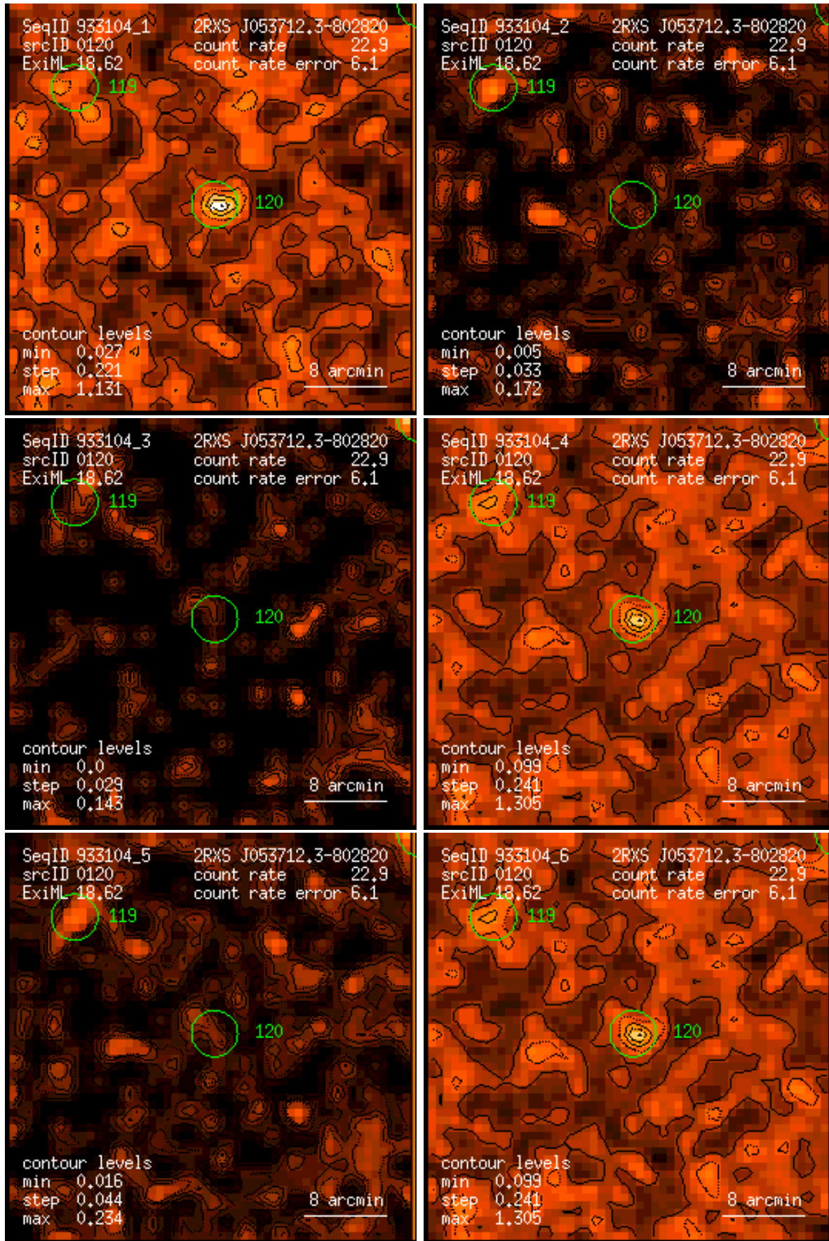
Figure 120: RASS 933104: detection 0120: band rate images, Gaussian filter: (1) PSPC channels 11 – 41, (2) 52 – 90, (3) 91 – 201, (4) 11 – 235, (5) 52 – 201, (6) 11 – 201. Broad band rates in counts/ks. Band rate contour levels in counts/ks/arcmin 2 .
