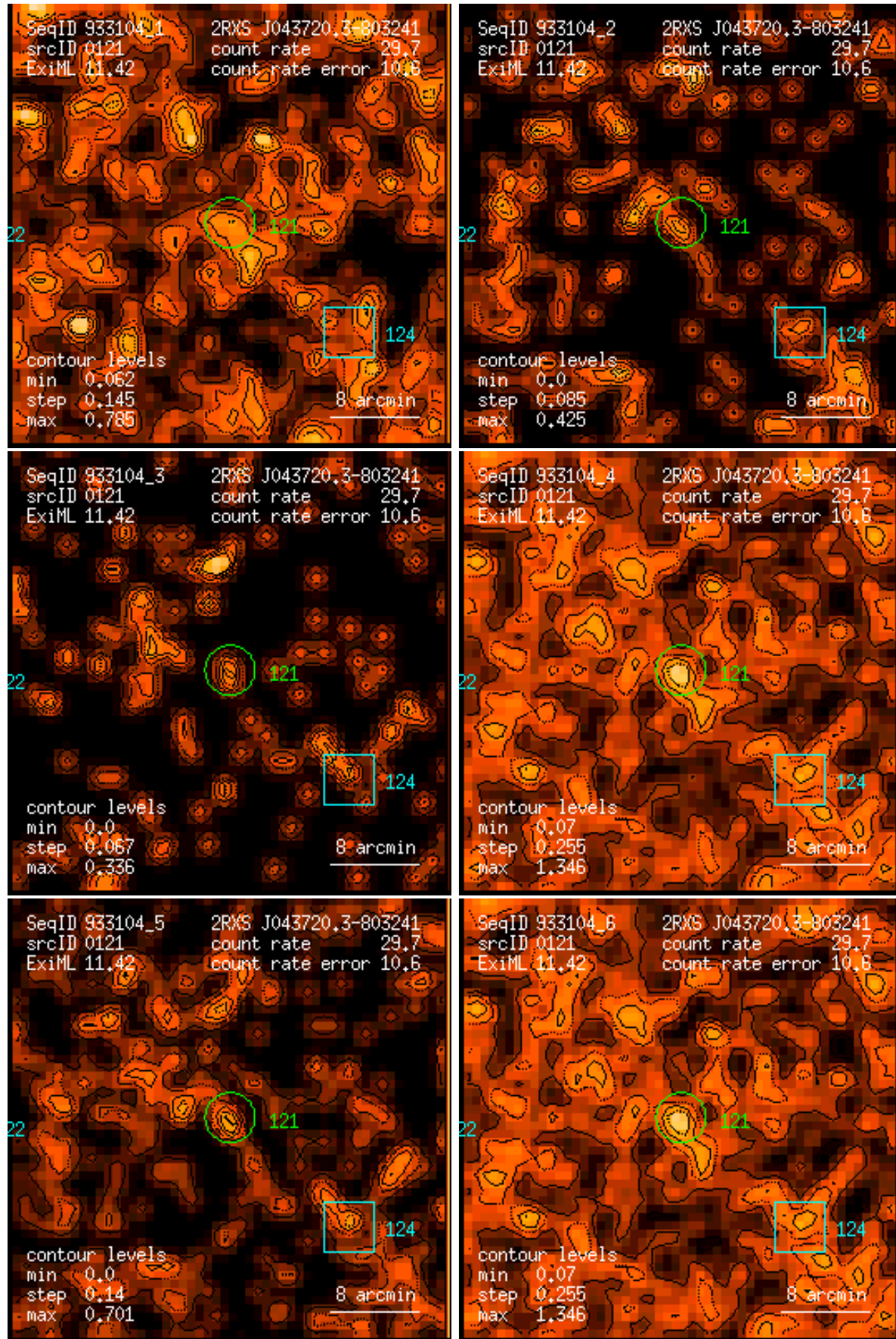
Figure 121: RASS 933104: detection 0121: band rate images, Gaussian filter: (1) PSPC channels 11 – 41, (2) 52 – 90, (3) 91 – 201, (4) 11 – 235, (5) 52 – 201, (6) 11 – 201. Broad band rates in counts/ks. Band rate contour levels in counts/ks/arcmin 2 .
