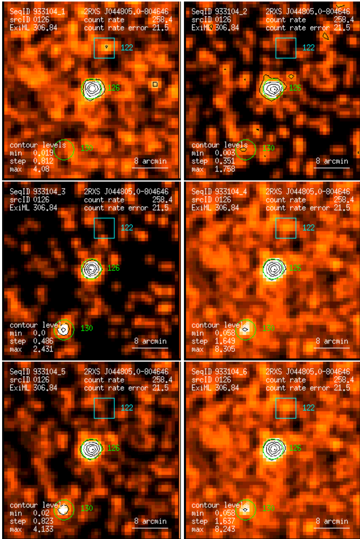
Figure 126: RASS 933104: detection 0126: band rate images, Gaussian filter: (1) PSPC channels 11 – 41, (2) 52 – 90, (3) 91 – 201, (4) 11 – 235, (5) 52 – 201, (6) 11 – 201. Broad band rates in counts/ks. Band rate contour levels in counts/ks/arcmin 2 .
