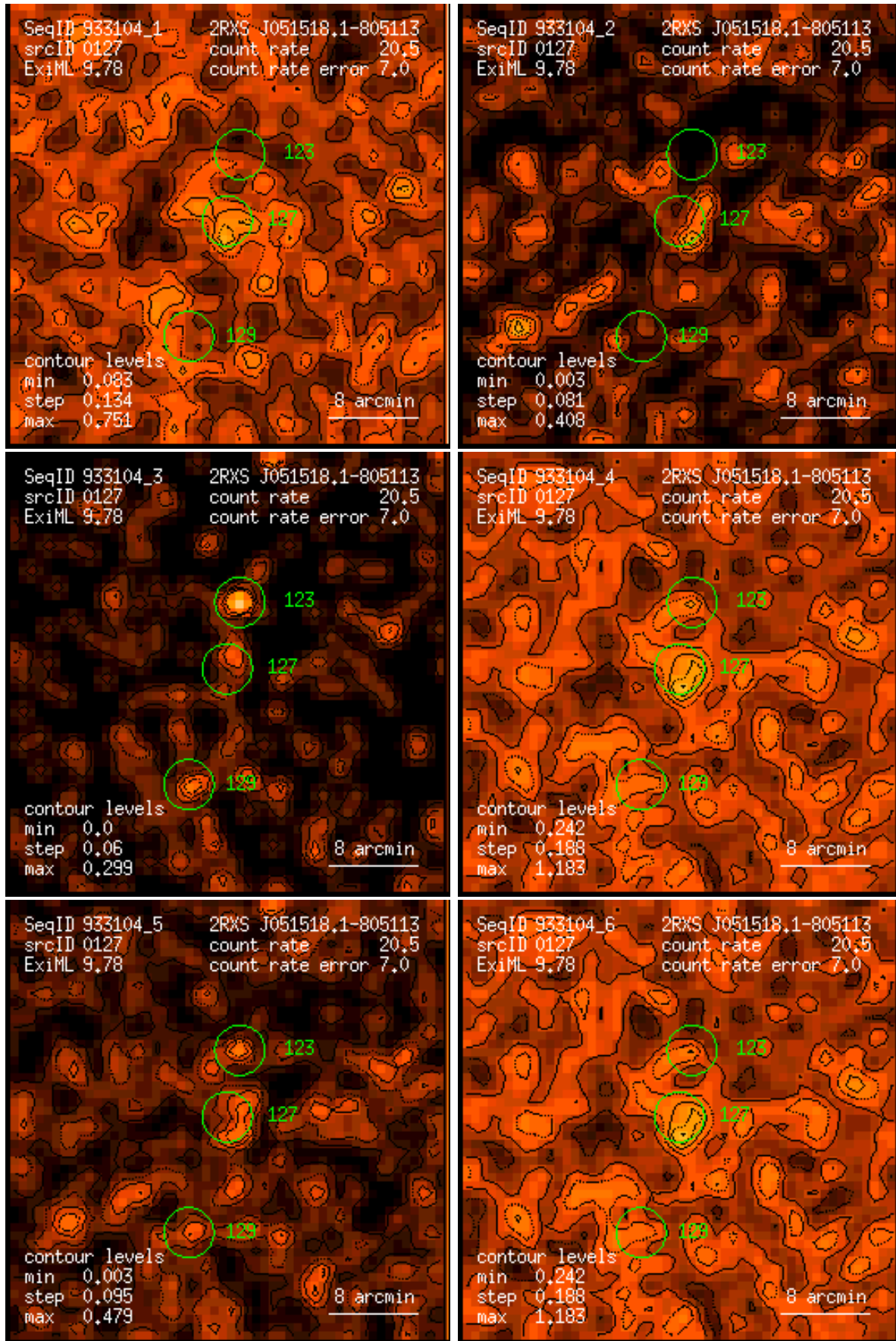
Figure 127: RASS 933104: detection 0127: band rate images, Gaussian filter: (1) PSPC channels 11 – 41, (2) 52 – 90, (3) 91 – 201, (4) 11 – 235, (5) 52 – 201, (6) 11 – 201. Broad band rates in counts/ks. Band rate contour levels in counts/ks/arcmin 2 .
