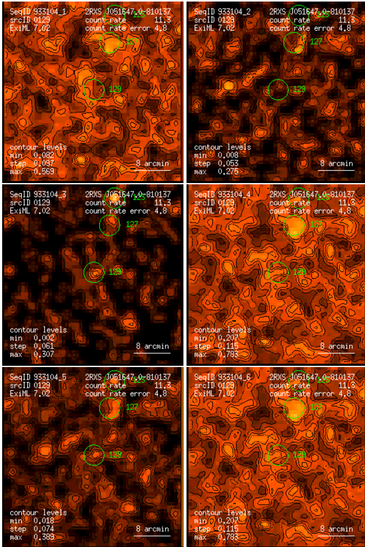
Figure 129: RASS 933104: detection 0129: band rate images, Gaussian filter: (1) PSPC channels 11 – 41, (2) 52 – 90, (3) 91 – 201, (4) 11 – 235, (5) 52 – 201, (6) 11 – 201. Broad band rates in counts/ks. Band rate contour levels in counts/ks/arcmin 2 .
