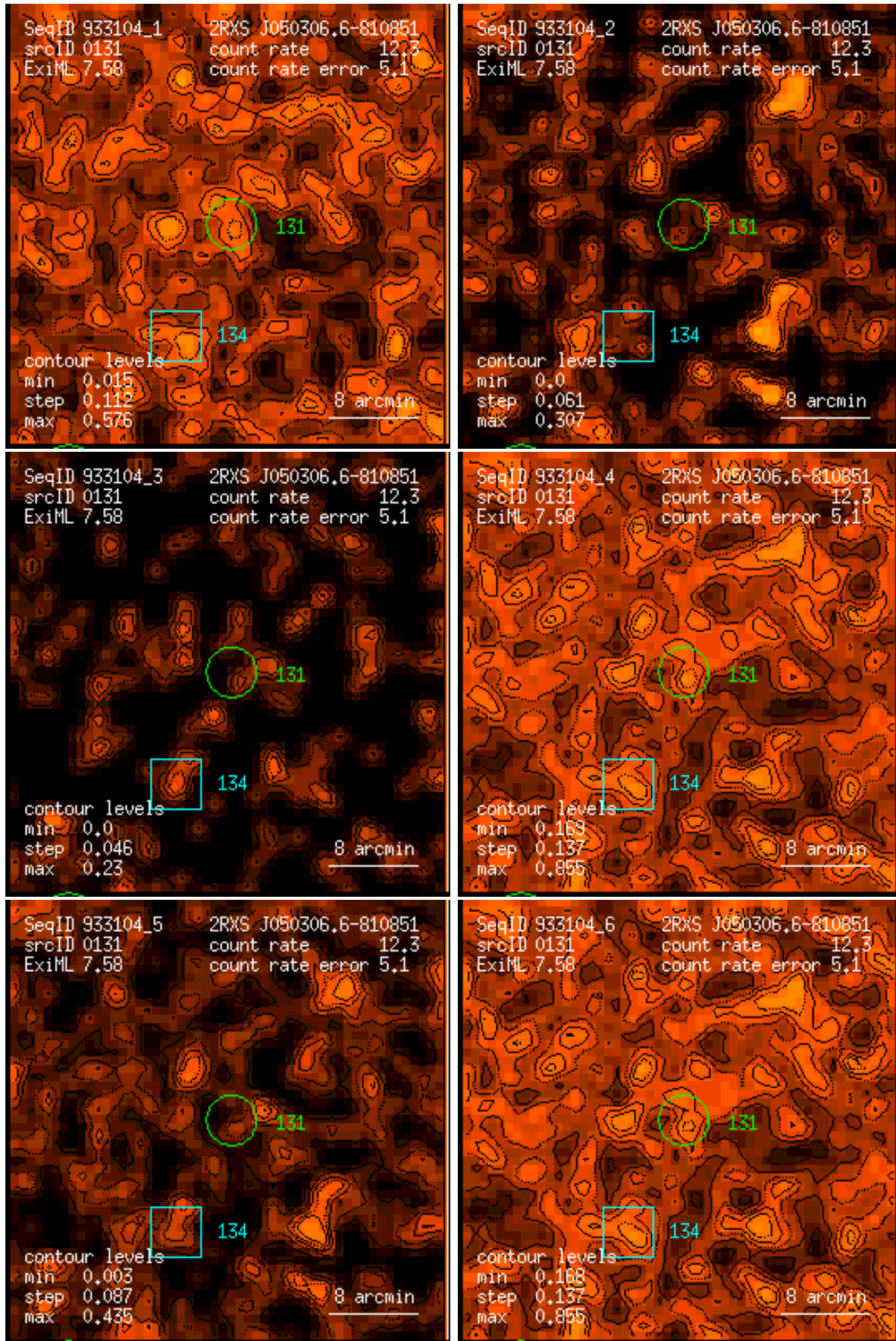
Figure 131: RASS 933104: detection 0131: band rate images, Gaussian filter: (1) PSPC channels 11 – 41, (2) 52 – 90, (3) 91 – 201, (4) 11 – 235, (5) 52 – 201, (6) 11 – 201. Broad band rates in counts/ks. Band rate contour levels in counts/ks/arcmin 2 .
