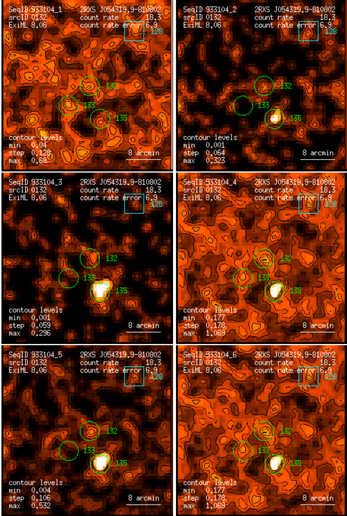
Figure 132: RASS 933104: detection 0132: band rate images, Gaussian filter: (1) PSPC channels 11 – 41, (2) 52 – 90, (3) 91 – 201, (4) 11 – 235, (5) 52 – 201, (6) 11 – 201. Broad band rates in counts/ks. Band rate contour levels in counts/ks/arcmin 2 .
