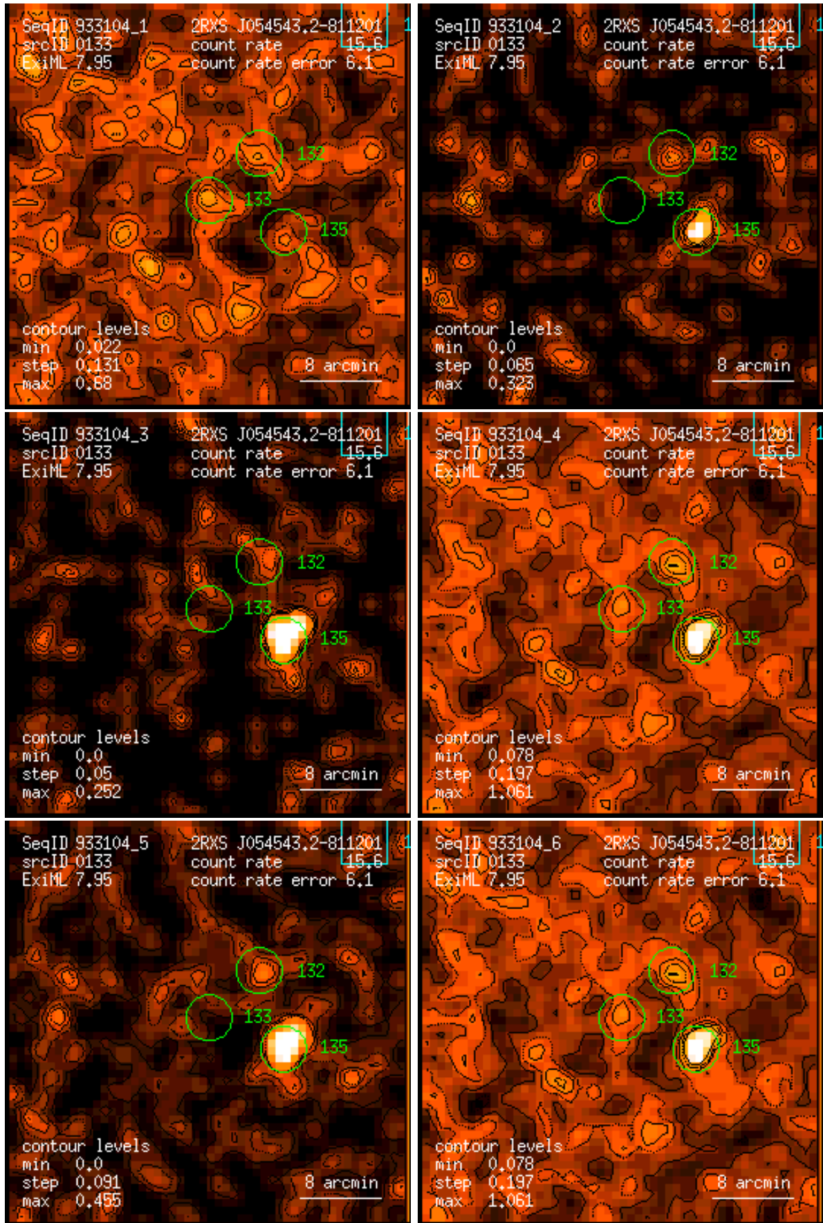
Figure 133: RASS 933104: detection 0133: band rate images, Gaussian filter: (1) PSPC channels 11 – 41, (2) 52 – 90, (3) 91 – 201, (4) 11 – 235, (5) 52 – 201, (6) 11 – 201. Broad band rates in counts/ks. Band rate contour levels in counts/ks/arcmin 2 .
