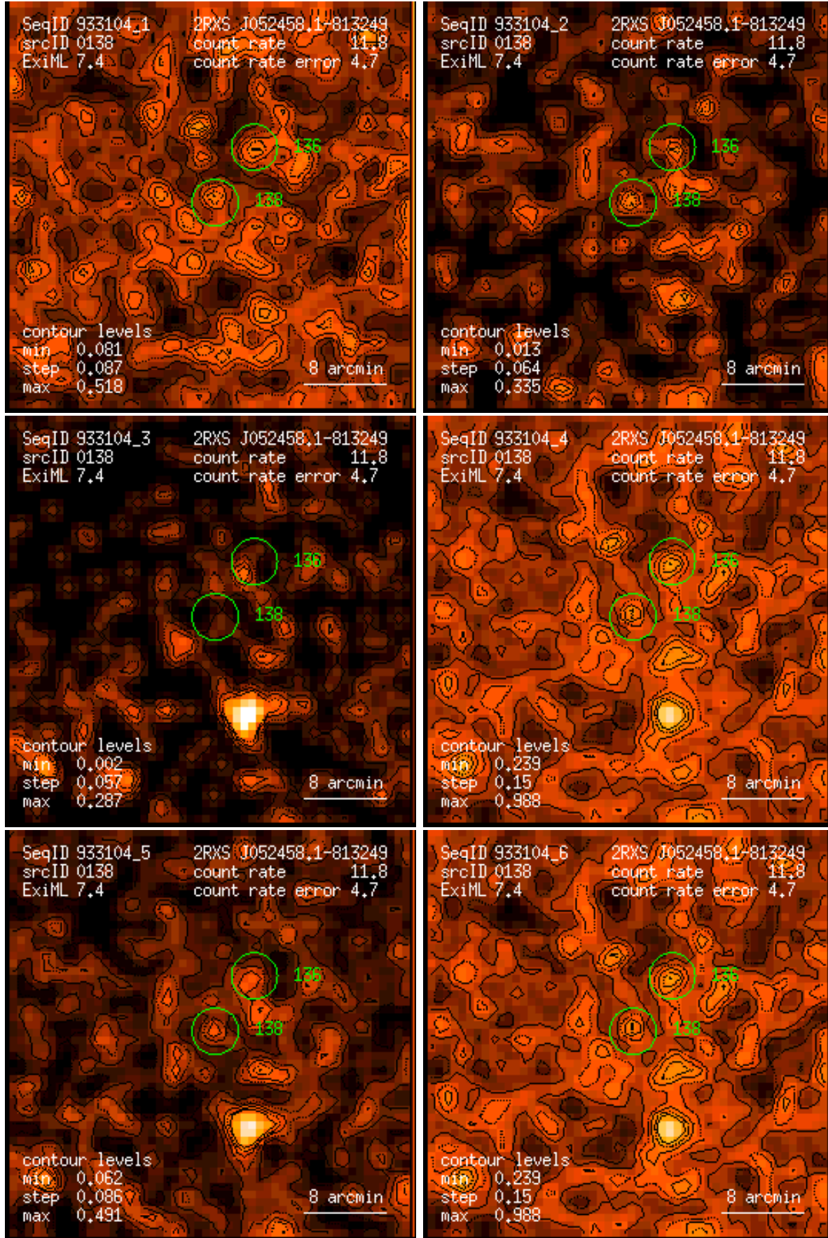
Figure 138: RASS 933104: detection 0138: band rate images, Gaussian filter: (1) PSPC channels 11 – 41, (2) 52 – 90, (3) 91 – 201, (4) 11 – 235, (5) 52 – 201, (6) 11 – 201. Broad band rates in counts/ks. Band rate contour levels in counts/ks/arcmin 2 .
