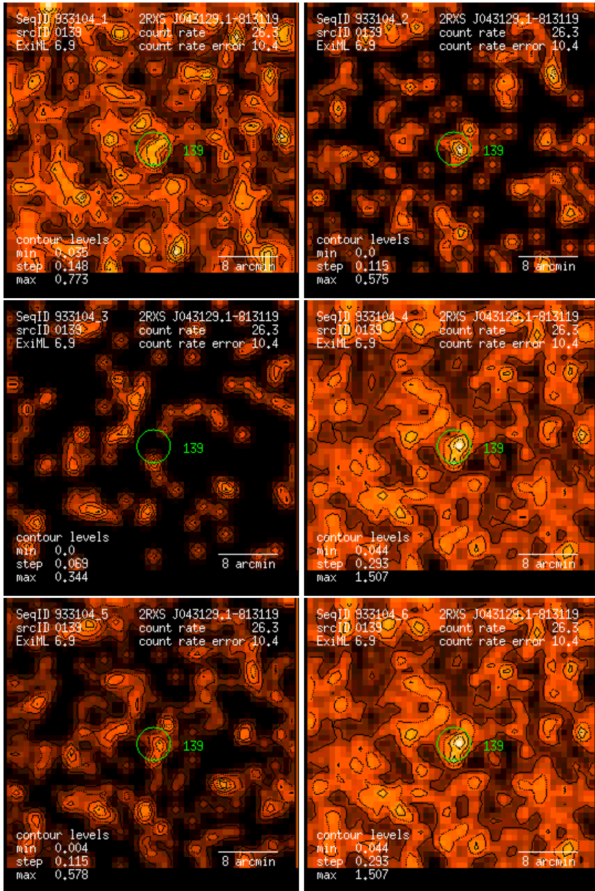
Figure 139: RASS 933104: detection 0139: band rate images, Gaussian filter: (1) PSPC channels 11 – 41, (2) 52 – 90, (3) 91 – 201, (4) 11 – 235, (5) 52 – 201, (6) 11 – 201. Broad band rates in counts/ks. Band rate contour levels in counts/ks/arcmin 2 .
