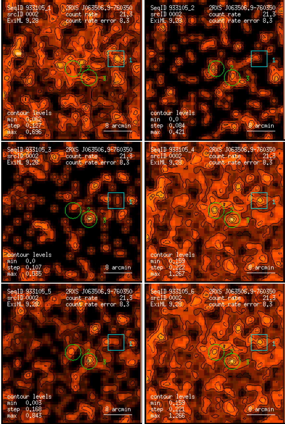
Figure 2: RASS 933105: detection 0002: band rate images, Gaussian filter: (1) PSPC channels 11 – 41, (2) 52 – 90, (3) 91 – 201, (4) 11 – 235, (5) 52 – 201, (6) 11 – 201. Broad band rates in counts/ks. Band rate contour levels in counts/ks/arcmin 2 .
