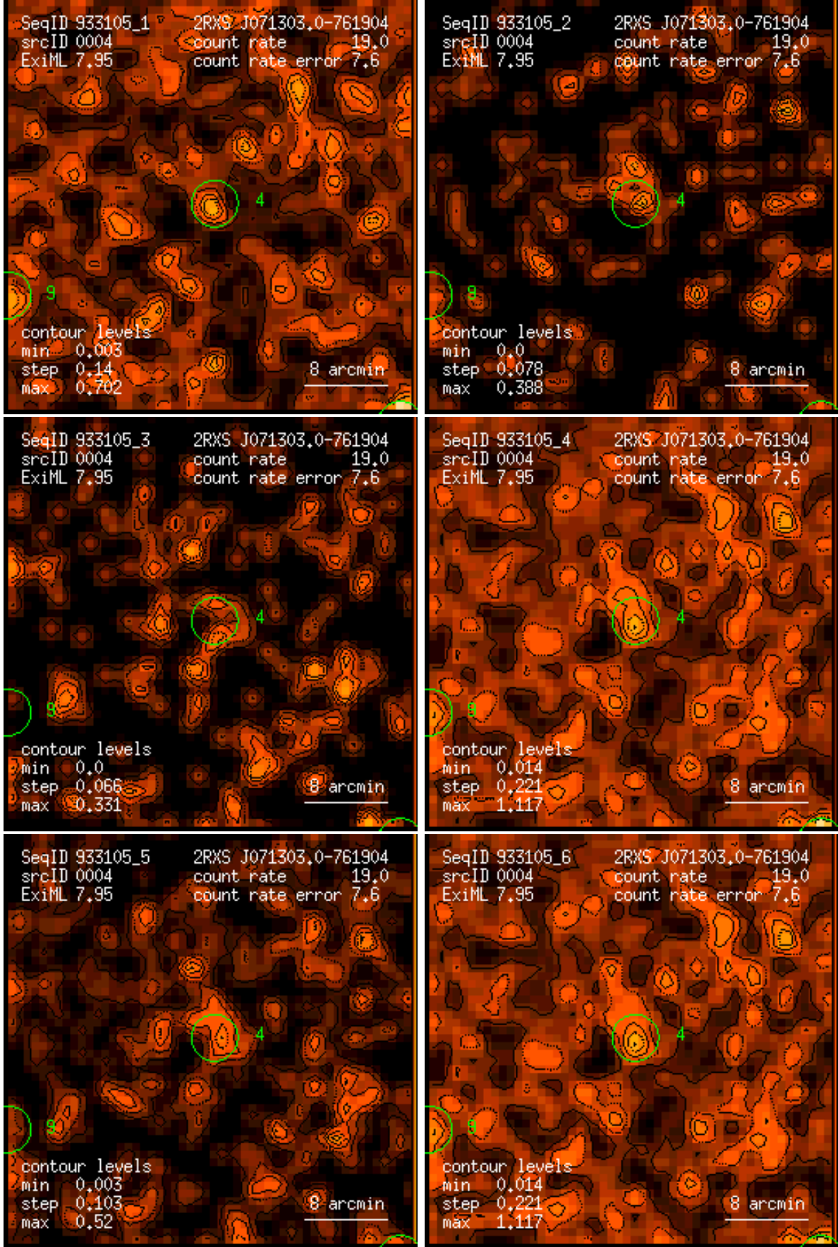
Figure 4: RASS 933105: detection 0004: band rate images, Gaussian filter: (1) PSPC channels 11 – 41, (2) 52 – 90, (3) 91 – 201, (4) 11 – 235, (5) 52 – 201, (6) 11 – 201. Broad band rates in counts/ks. Band rate contour levels in counts/ks/arcmin 2 .
