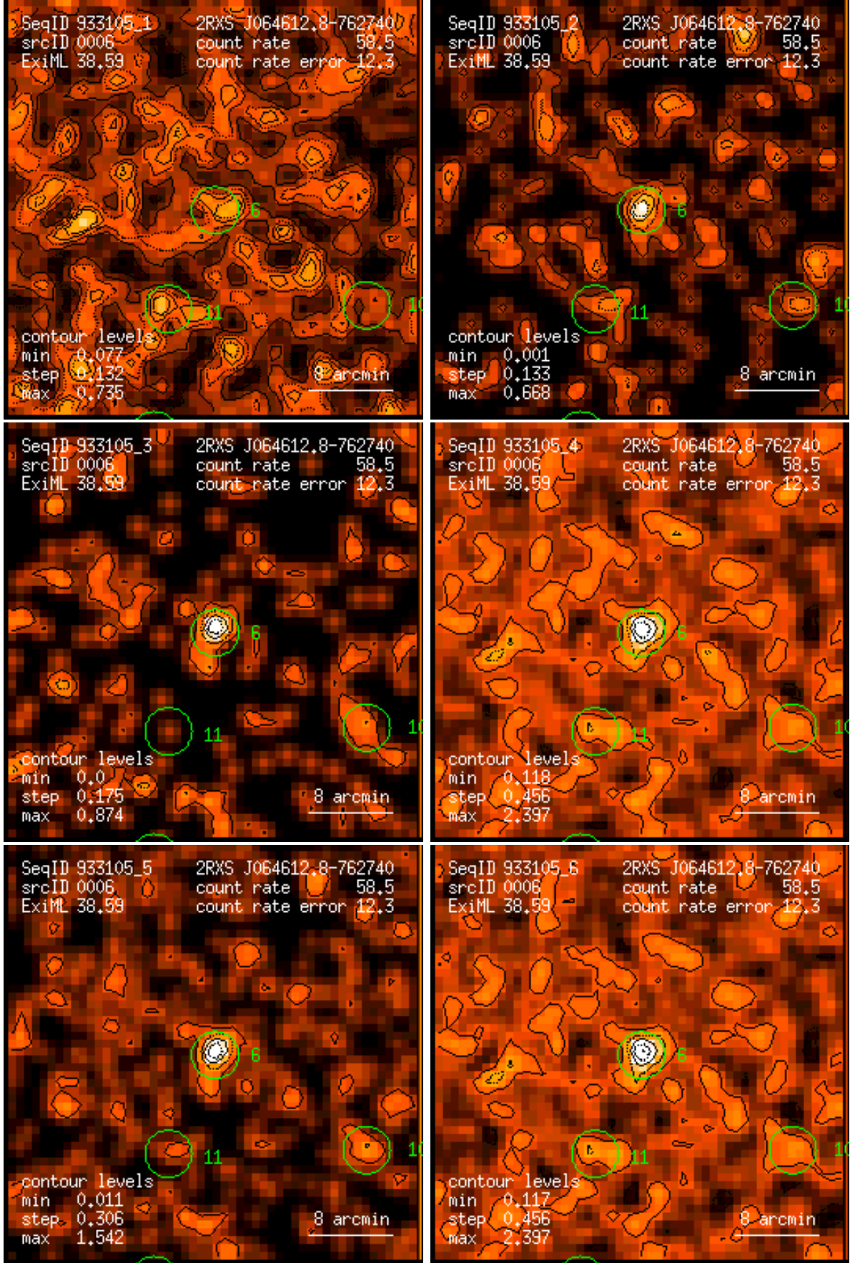
Figure 6: RASS 933105: detection 0006: band rate images, Gaussian filter: (1) PSPC channels 11 – 41, (2) 52 – 90, (3) 91 – 201, (4) 11 – 235, (5) 52 – 201, (6) 11 – 201. Broad band rates in counts/ks. Band rate contour levels in counts/ks/arcmin 2 .
