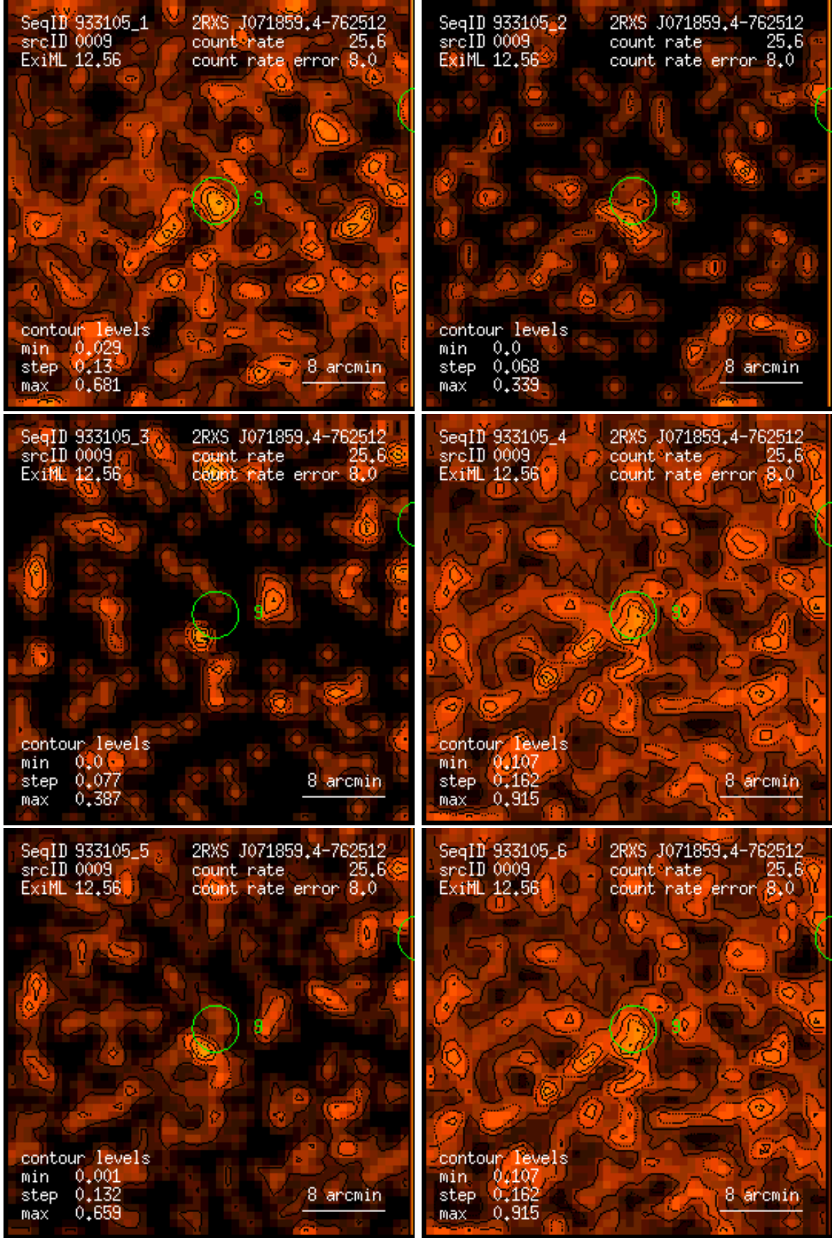
Figure 9: RASS 933105: detection 0009: band rate images, Gaussian filter: (1) PSPC channels 11 – 41, (2) 52 – 90, (3) 91 – 201, (4) 11 – 235, (5) 52 – 201, (6) 11 – 201. Broad band rates in counts/ks. Band rate contour levels in counts/ks/arcmin 2 .
