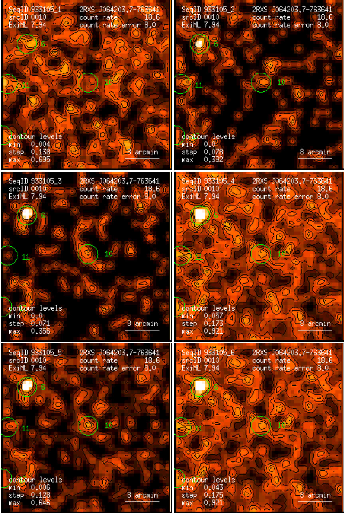
Figure 10: RASS 933105: detection 0010: band rate images, Gaussian filter: (1) PSPC channels 11 – 41, (2) 52 – 90, (3) 91 – 201, (4) 11 – 235, (5) 52 – 201, (6) 11 – 201. Broad band rates in counts/ks. Band rate contour levels in counts/ks/arcmin 2 .
