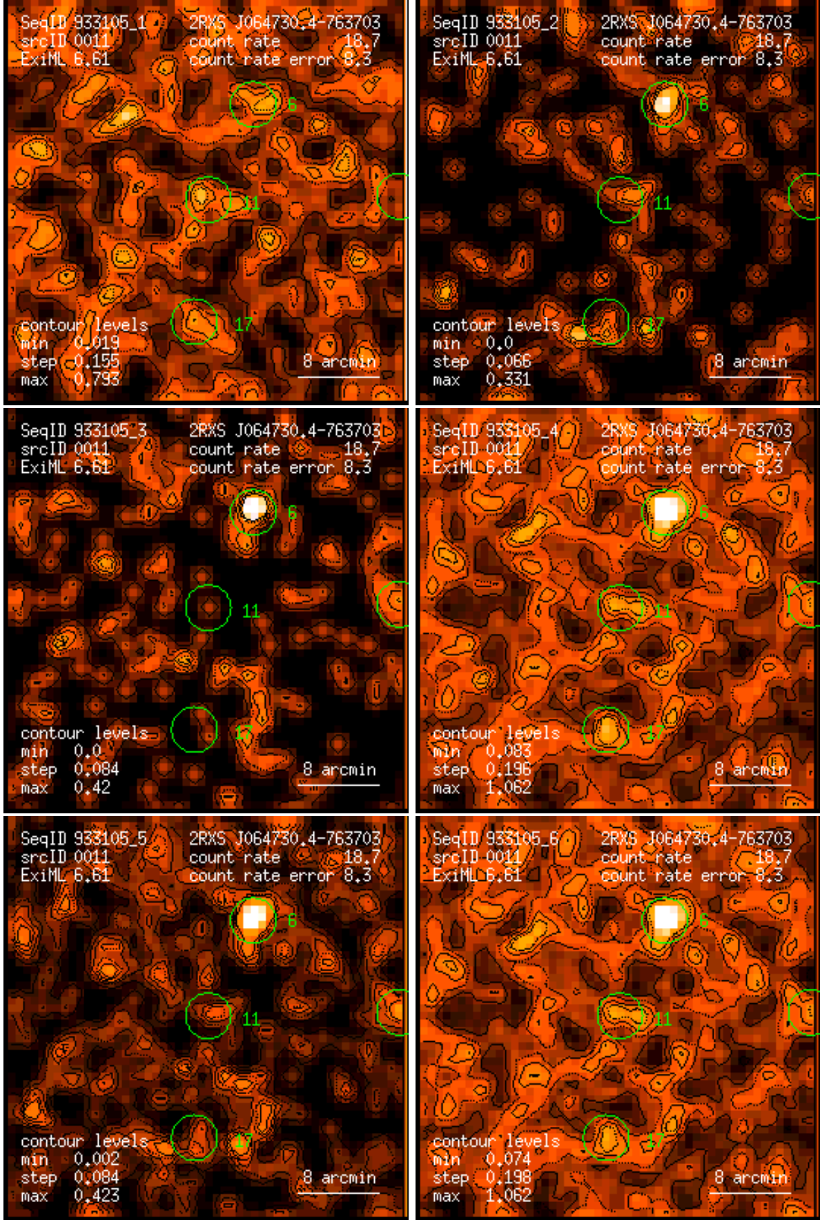
Figure 11: RASS 933105: detection 0011: band rate images, Gaussian filter: (1) PSPC channels 11 – 41, (2) 52 – 90, (3) 91 – 201, (4) 11 – 235, (5) 52 – 201, (6) 11 – 201. Broad band rates in counts/ks. Band rate contour levels in counts/ks/arcmin 2 .
