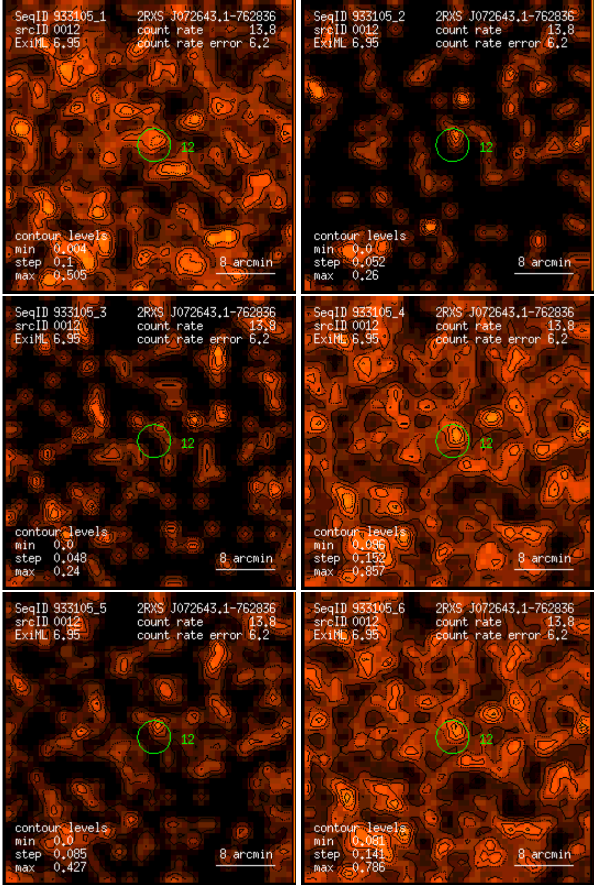
Figure 12: RASS 933105: detection 0012: band rate images, Gaussian filter: (1) PSPC channels 11 – 41, (2) 52 – 90, (3) 91 – 201, (4) 11 – 235, (5) 52 – 201, (6) 11 – 201. Broad band rates in counts/ks. Band rate contour levels in counts/ks/arcmin 2 .
