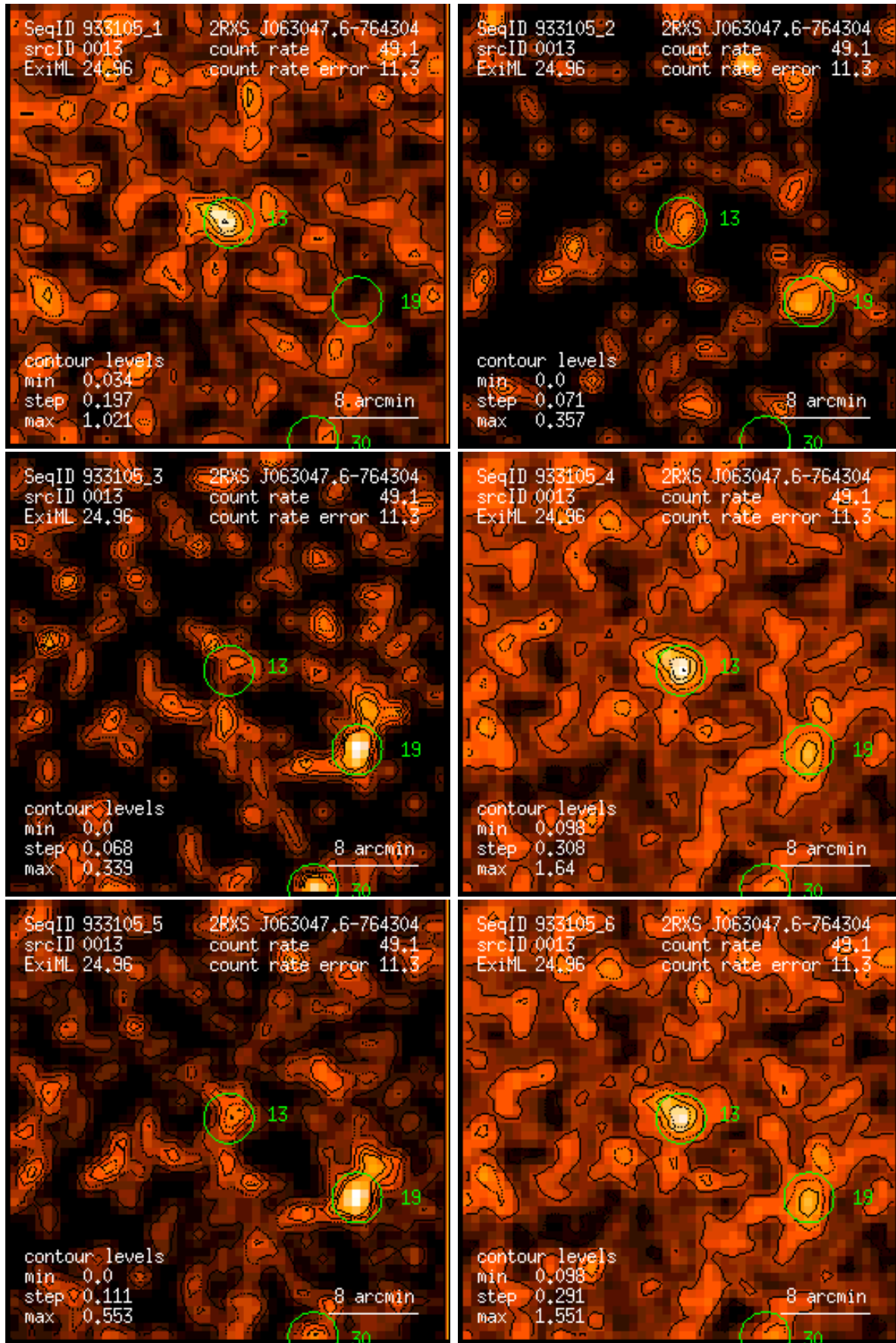
Figure 13: RASS 933105: detection 0013: band rate images, Gaussian filter: (1) PSPC channels 11 – 41, (2) 52 – 90, (3) 91 – 201, (4) 11 – 235, (5) 52 – 201, (6) 11 – 201. Broad band rates in counts/ks. Band rate contour levels in counts/ks/arcmin 2 .
