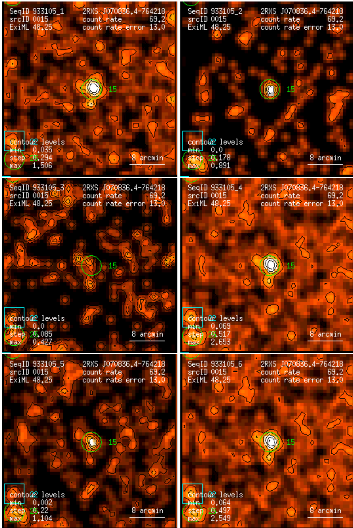
Figure 15: RASS 933105: detection 0015: band rate images, Gaussian filter: (1) PSPC channels 11 – 41, (2) 52 – 90, (3) 91 – 201, (4) 11 – 235, (5) 52 – 201, (6) 11 – 201. Broad band rates in counts/ks. Band rate contour levels in counts/ks/arcmin 2 .
