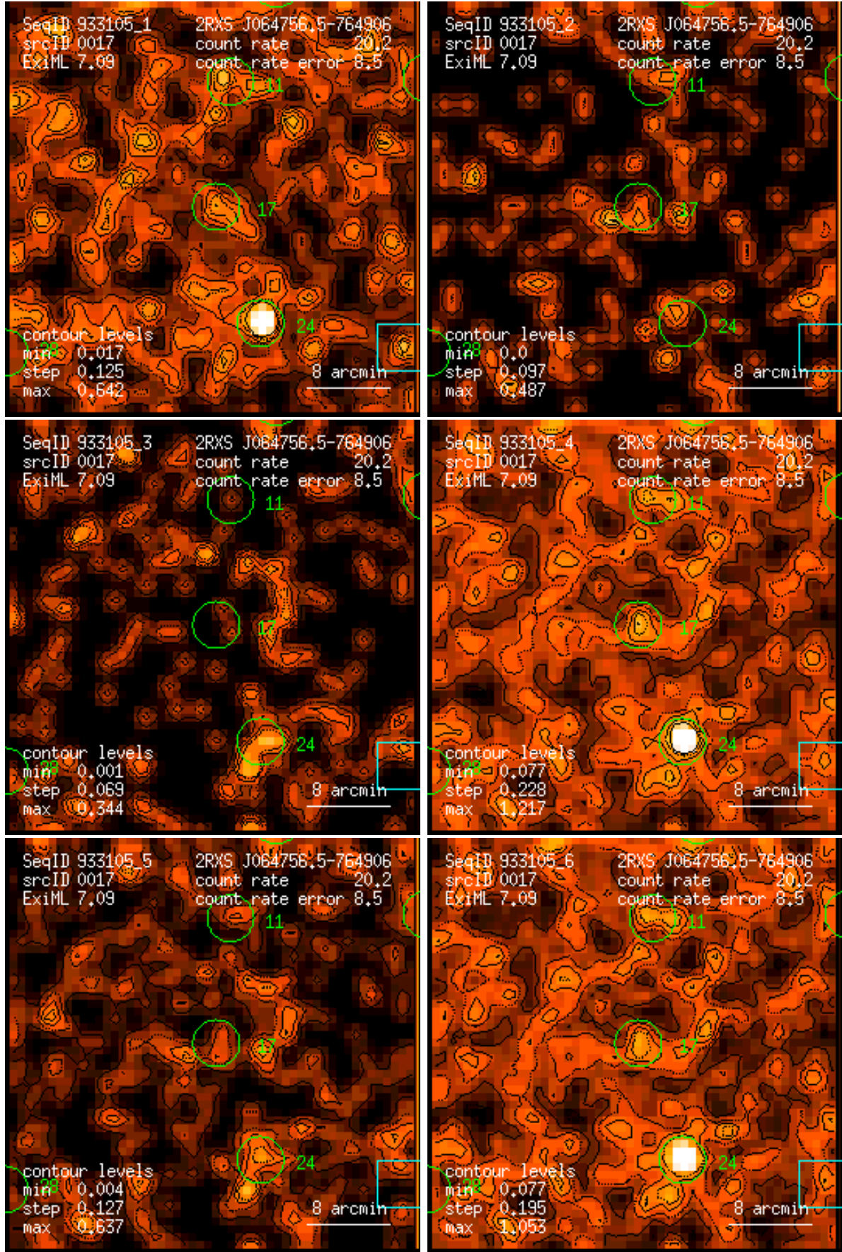
Figure 17: RASS 933105: detection 0017: band rate images, Gaussian filter: (1) PSPC channels 11 – 41, (2) 52 – 90, (3) 91 – 201, (4) 11 – 235, (5) 52 – 201, (6) 11 – 201. Broad band rates in counts/ks. Band rate contour levels in counts/ks/arcmin 2 .
