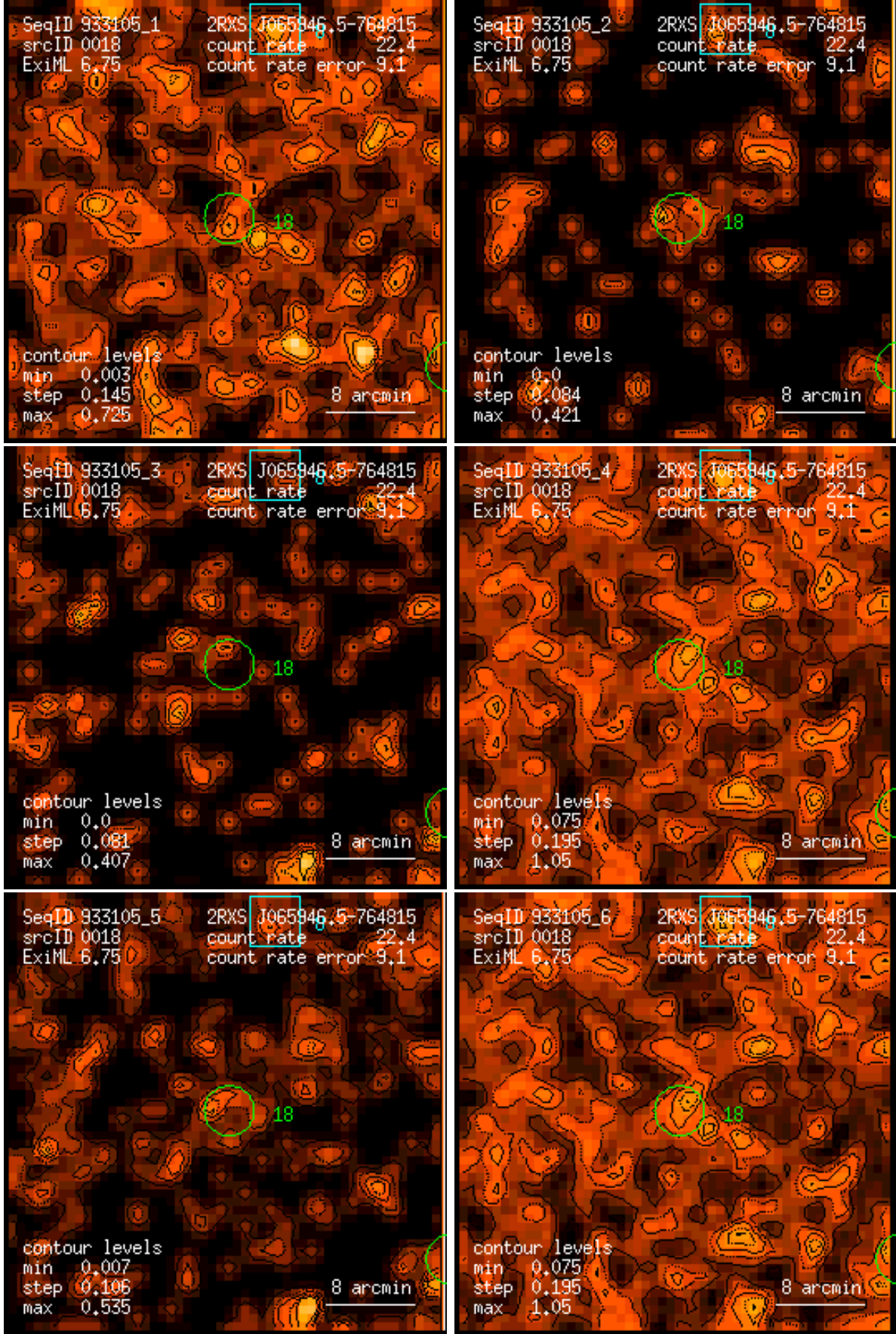
Figure 18: RASS 933105: detection 0018: band rate images, Gaussian filter: (1) PSPC channels 11 – 41, (2) 52 – 90, (3) 91 – 201, (4) 11 – 235, (5) 52 – 201, (6) 11 – 201. Broad band rates in counts/ks. Band rate contour levels in counts/ks/arcmin 2 .
