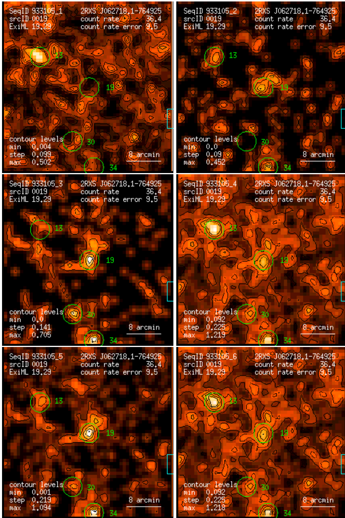
Figure 19: RASS 933105: detection 0019: band rate images, Gaussian filter: (1) PSPC channels 11 – 41, (2) 52 – 90, (3) 91 – 201, (4) 11 – 235, (5) 52 – 201, (6) 11 – 201. Broad band rates in counts/ks. Band rate contour levels in counts/ks/arcmin 2 .
