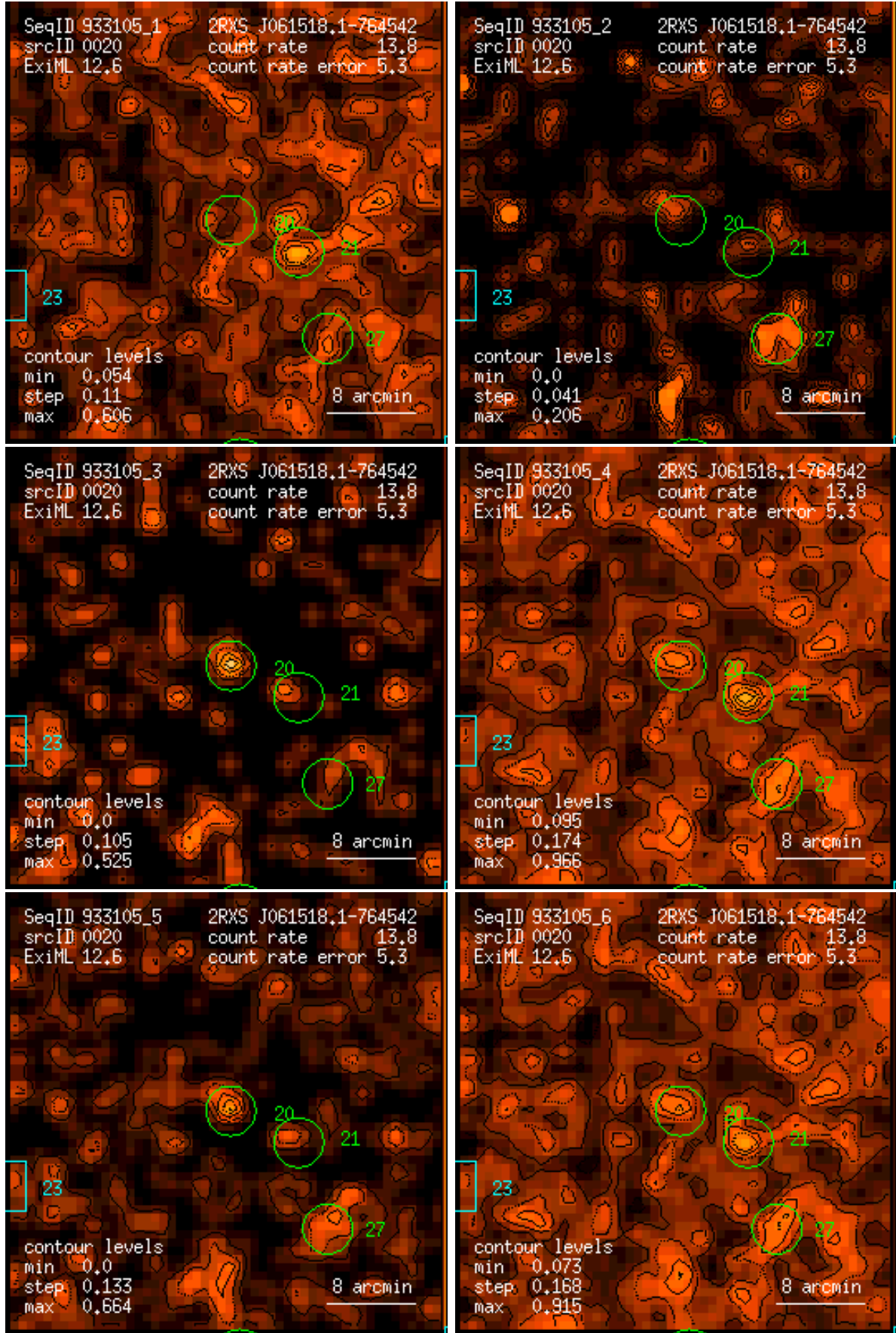
Figure 20: RASS 933105: detection 0020: band rate images, Gaussian filter: (1) PSPC channels 11 – 41, (2) 52 – 90, (3) 91 – 201, (4) 11 – 235, (5) 52 – 201, (6) 11 – 201. Broad band rates in counts/ks. Band rate contour levels in counts/ks/arcmin 2 .
