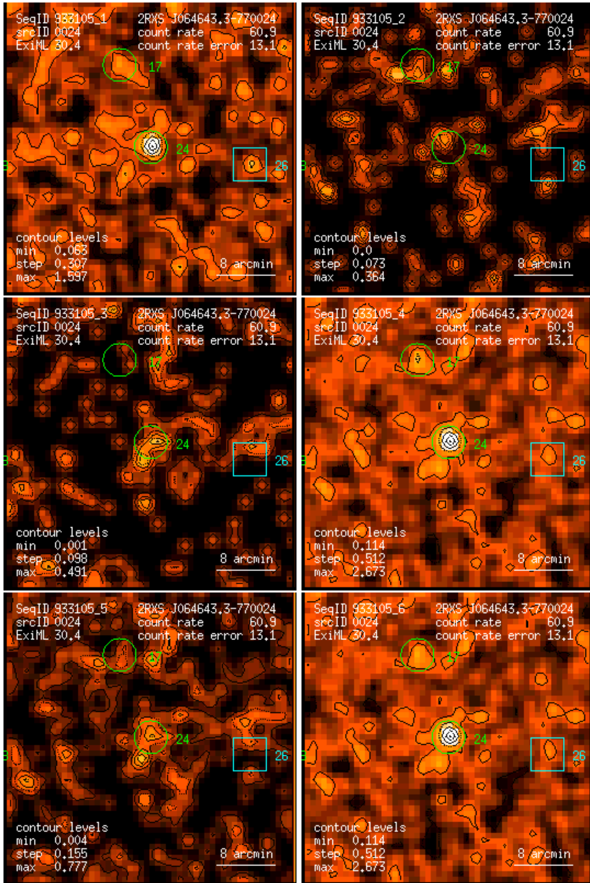
Figure 24: RASS 933105: detection 0024: band rate images, Gaussian filter: (1) PSPC channels 11 – 41, (2) 52 – 90, (3) 91 – 201, (4) 11 – 235, (5) 52 – 201, (6) 11 – 201. Broad band rates in counts/ks. Band rate contour levels in counts/ks/arcmin 2 .
