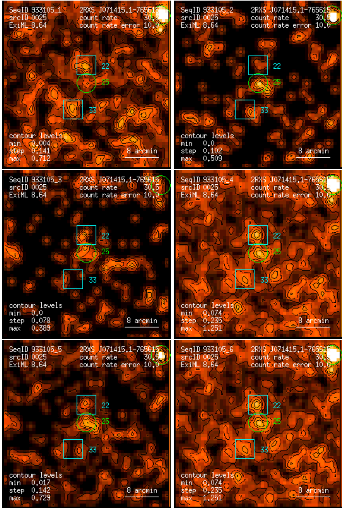
Figure 25: RASS 933105: detection 0025: band rate images, Gaussian filter: (1) PSPC channels 11 – 41, (2) 52 – 90, (3) 91 – 201, (4) 11 – 235, (5) 52 – 201, (6) 11 – 201. Broad band rates in counts/ks. Band rate contour levels in counts/ks/arcmin 2 .
