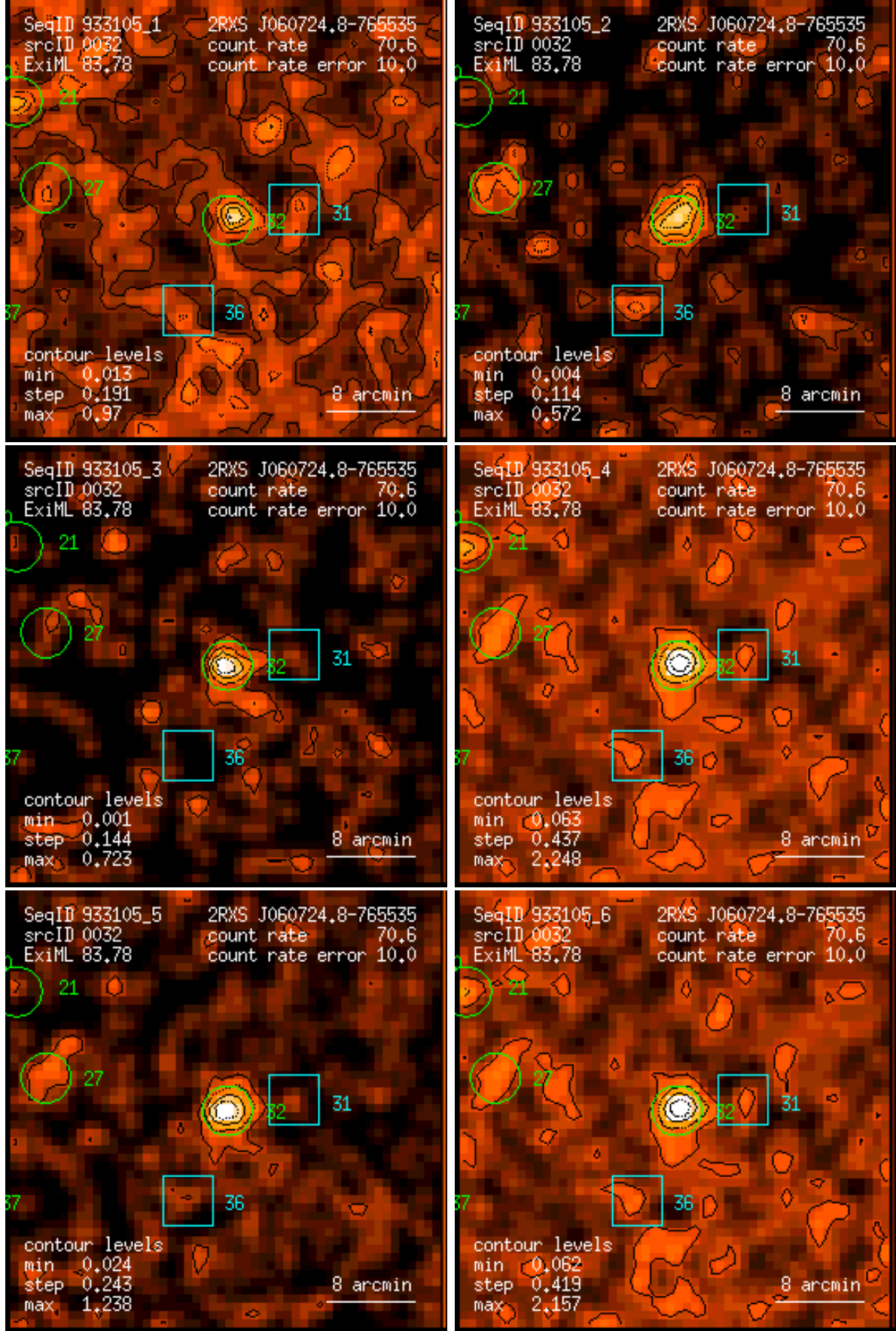
Figure 32: RASS 933105: detection 0032: band rate images, Gaussian filter: (1) PSPC channels 11 – 41, (2) 52 – 90, (3) 91 – 201, (4) 11 – 235, (5) 52 – 201, (6) 11 – 201. Broad band rates in counts/ks. Band rate contour levels in counts/ks/arcmin 2 .
