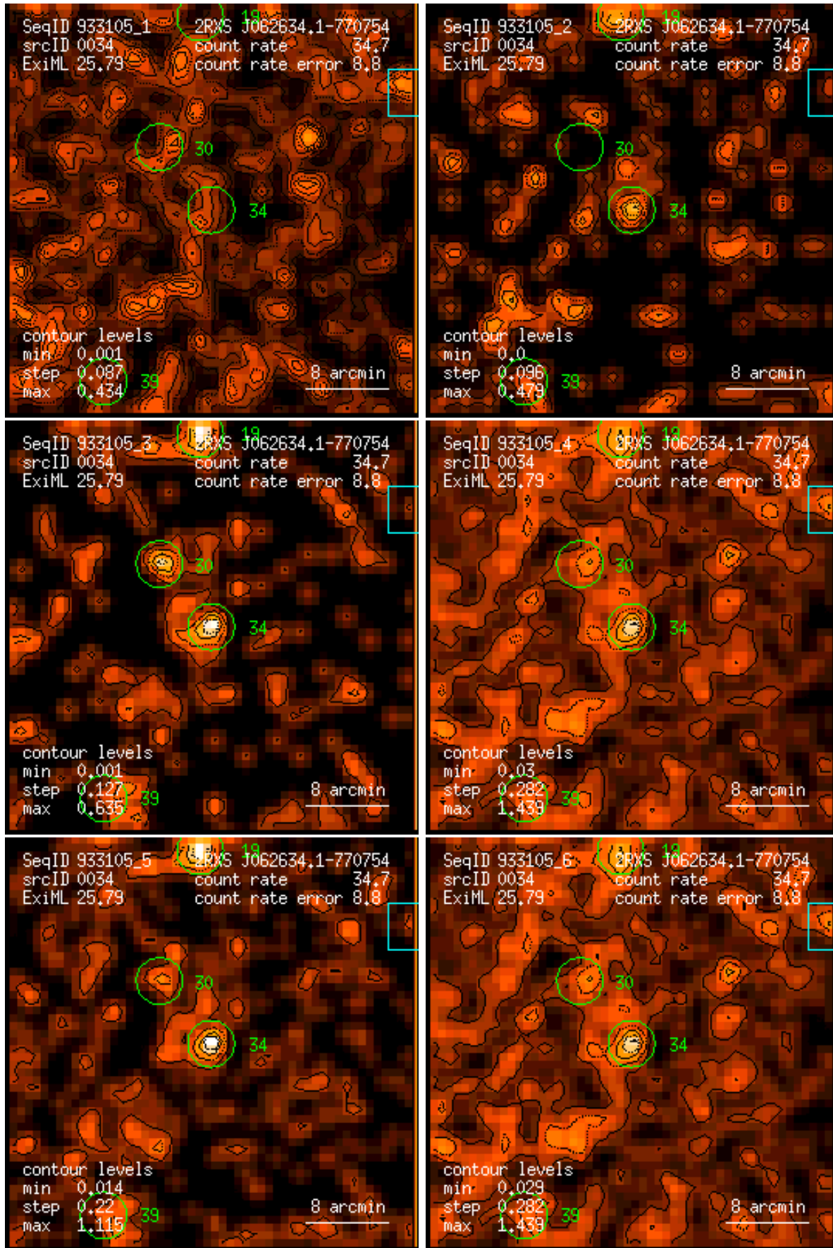
Figure 34: RASS 933105: detection 0034: band rate images, Gaussian filter: (1) PSPC channels 11 – 41, (2) 52 – 90, (3) 91 – 201, (4) 11 – 235, (5) 52 – 201, (6) 11 – 201. Broad band rates in counts/ks. Band rate contour levels in counts/ks/arcmin 2 .
