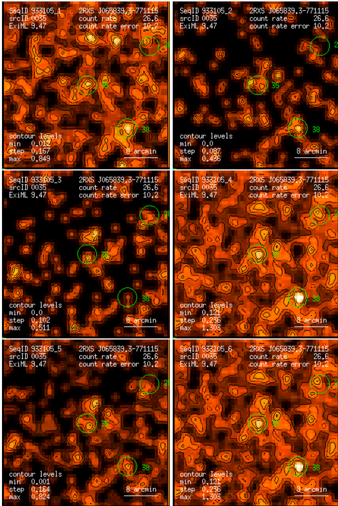
Figure 35: RASS 933105: detection 0035: band rate images, Gaussian filter: (1) PSPC channels 11 – 41, (2) 52 – 90, (3) 91 – 201, (4) 11 – 235, (5) 52 – 201, (6) 11 – 201. Broad band rates in counts/ks. Band rate contour levels in counts/ks/arcmin 2 .
