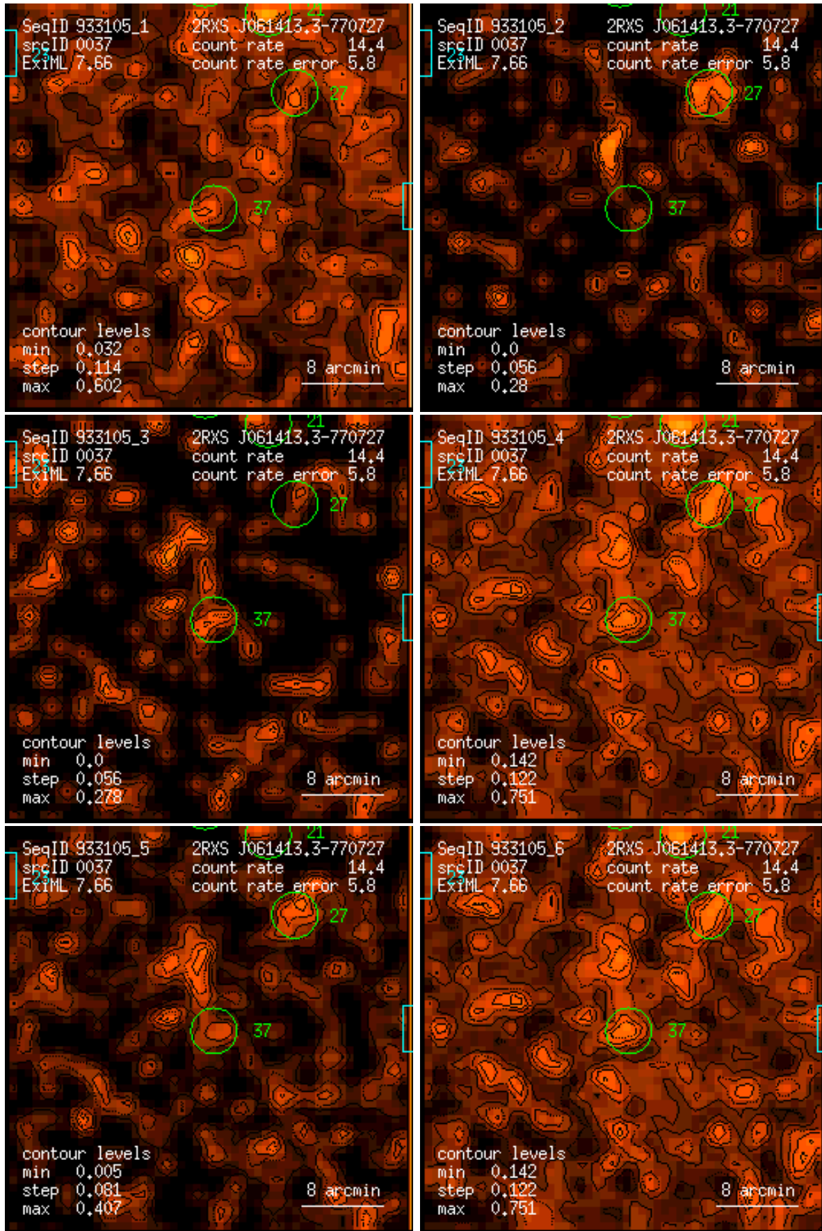
Figure 37: RASS 933105: detection 0037: band rate images, Gaussian filter: (1) PSPC channels 11 – 41, (2) 52 – 90, (3) 91 – 201, (4) 11 – 235, (5) 52 – 201, (6) 11 – 201. Broad band rates in counts/ks. Band rate contour levels in counts/ks/arcmin 2 .
