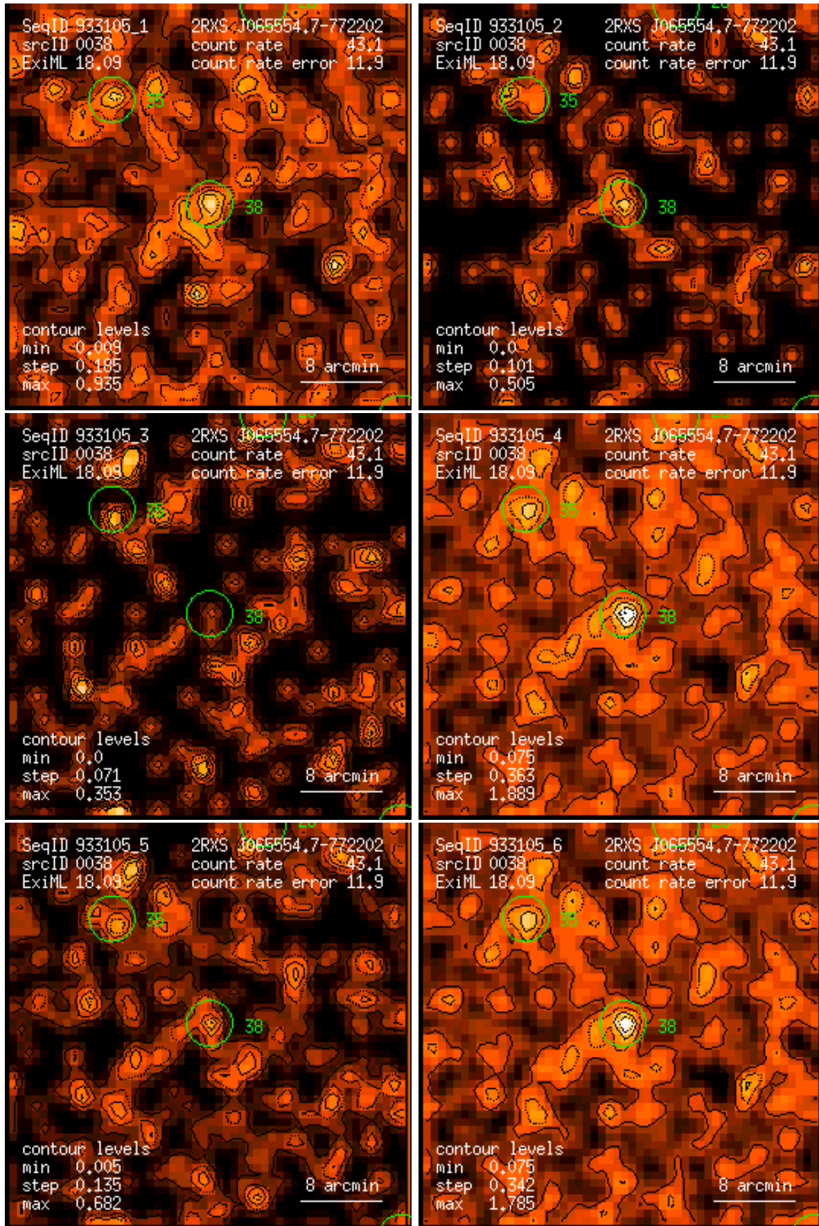
Figure 38: RASS 933105: detection 0038: band rate images, Gaussian filter: (1) PSPC channels 11 – 41, (2) 52 – 90, (3) 91 – 201, (4) 11 – 235, (5) 52 – 201, (6) 11 – 201. Broad band rates in counts/ks. Band rate contour levels in counts/ks/arcmin 2 .
