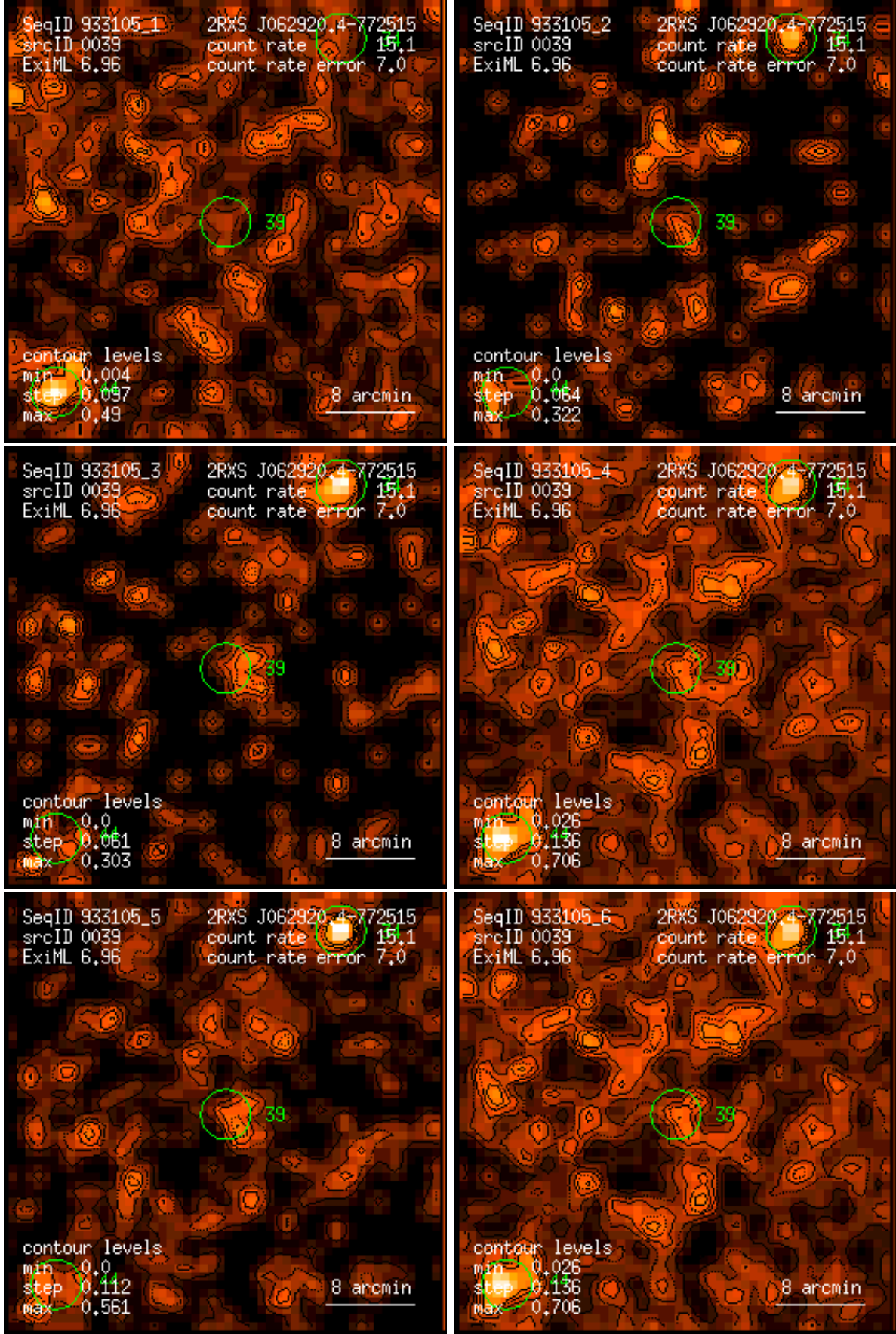
Figure 39: RASS 933105: detection 0039: band rate images, Gaussian filter: (1) PSPC channels 11 – 41, (2) 52 – 90, (3) 91 – 201, (4) 11 – 235, (5) 52 – 201, (6) 11 – 201. Broad band rates in counts/ks. Band rate contour levels in counts/ks/arcmin 2 .
